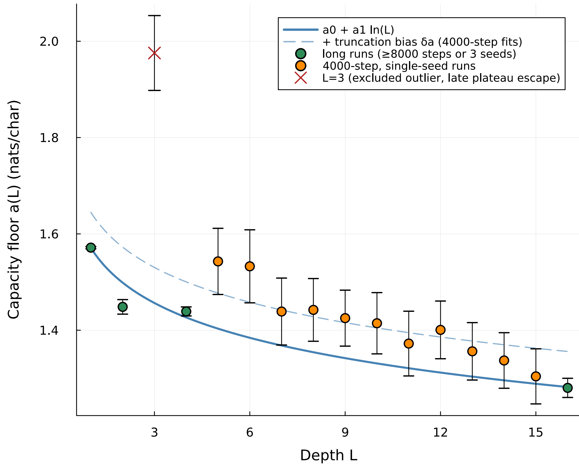
(a) Fitted capacity floor across 16 depths
