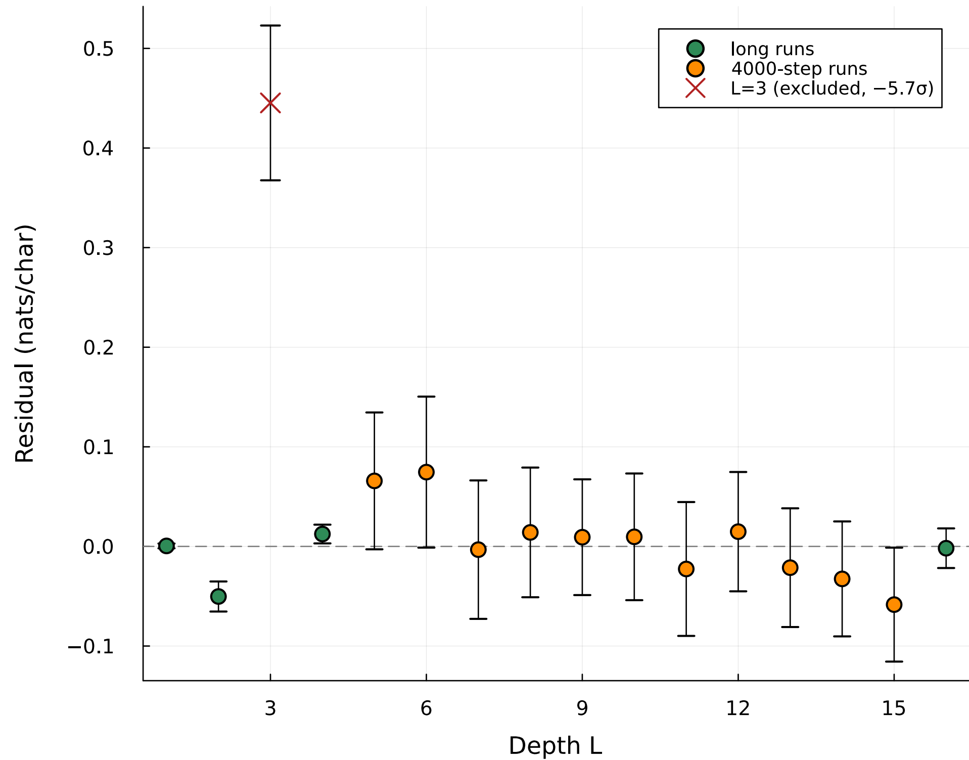
(b) Residuals vs. retained fit (incl. truncation-bias term)
