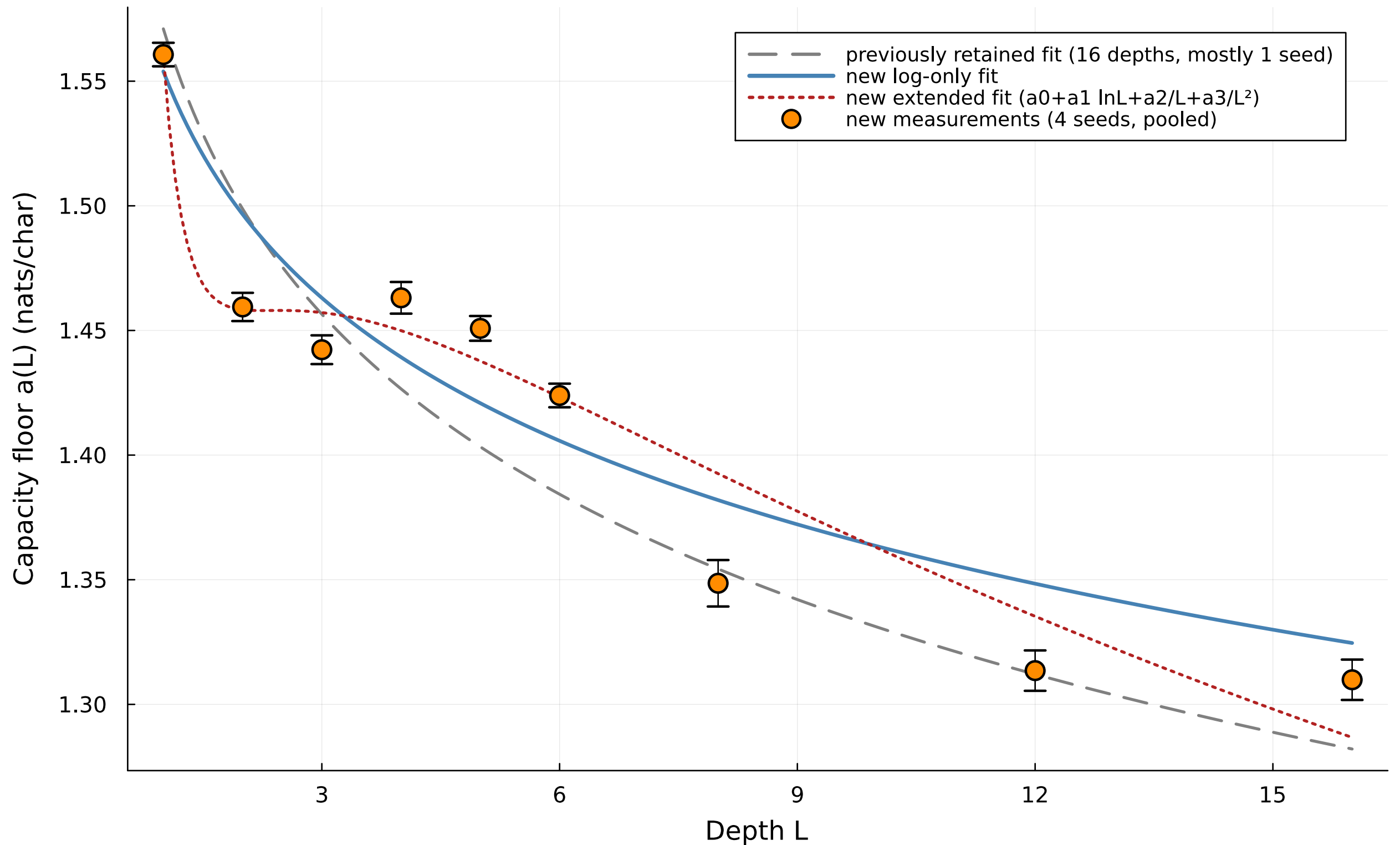
Constraint-test campaign: 9 depths, 4 seeds, long runs (20-40k steps)
