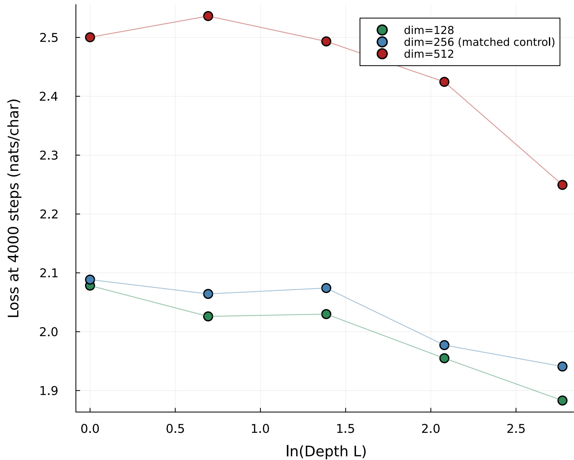
(a) Width sweep: dim=128/256/512
