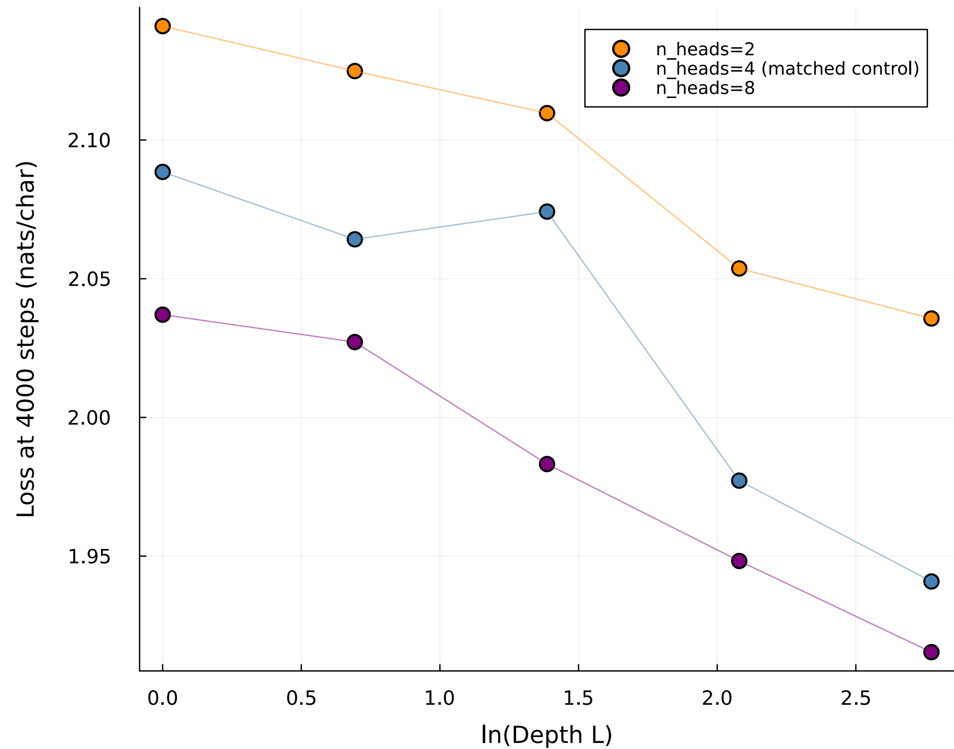
(b) Head-count sweep at dim=256 fixed
