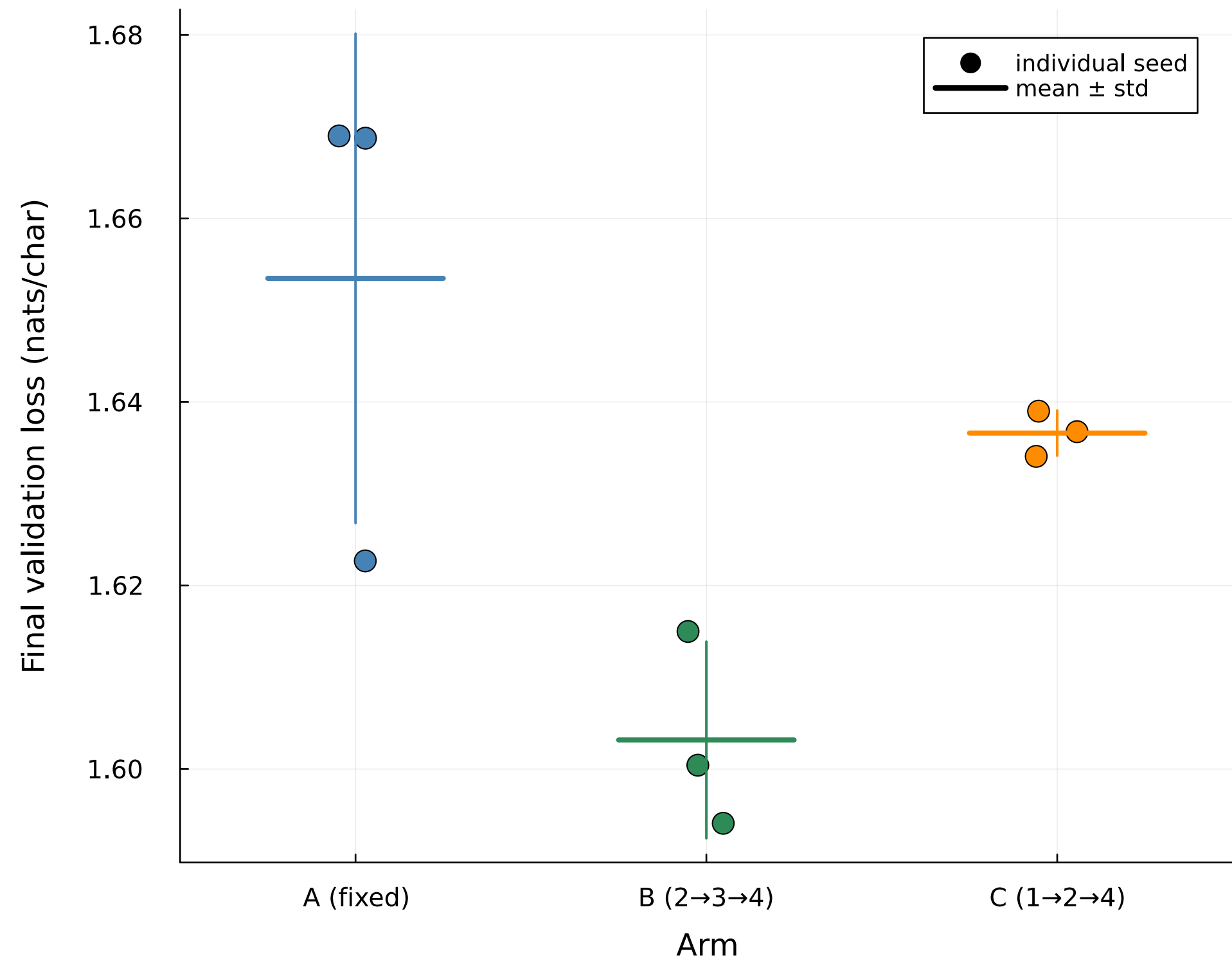
(b) Final val loss: 3 seeds per arm, equal FLOPs budget
