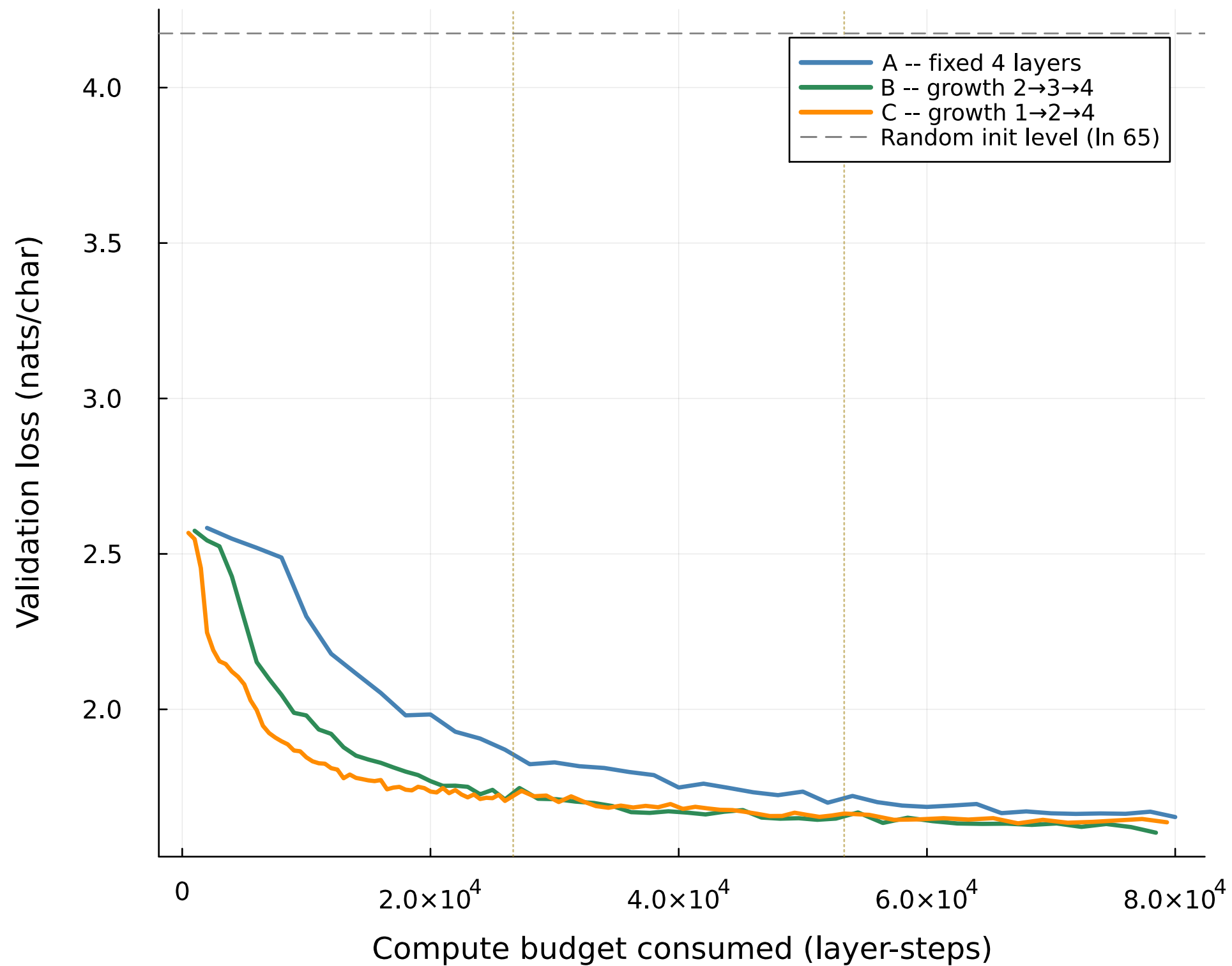
(a) Val loss vs. compute budget (mean of 3 seeds)
