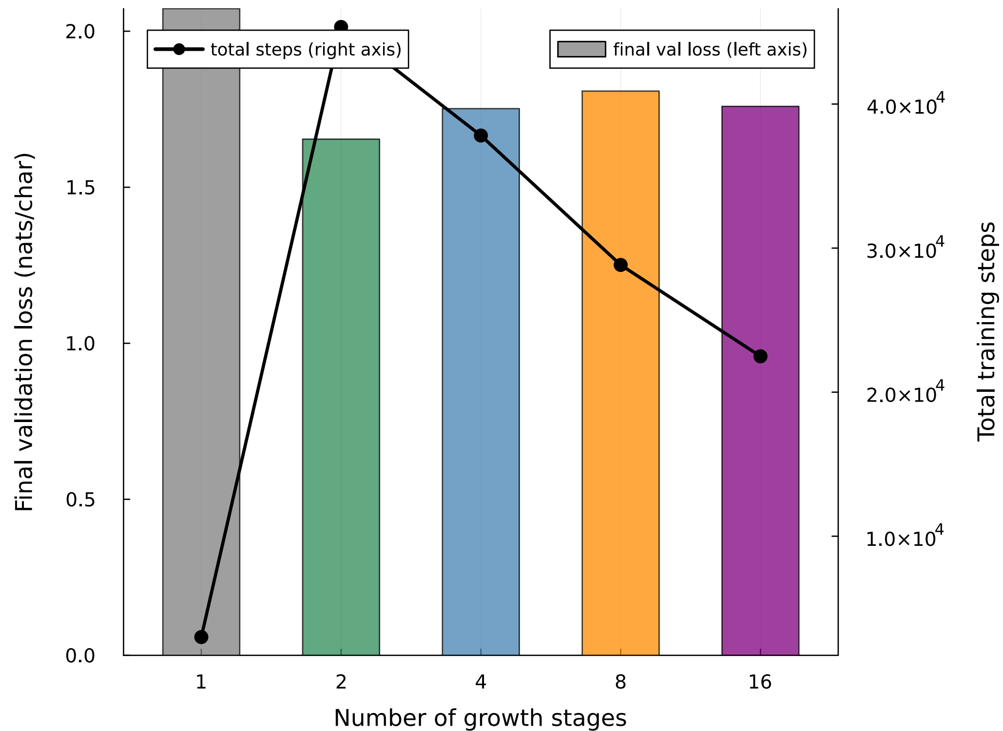
(b) Final loss and total steps vs. schedule density
