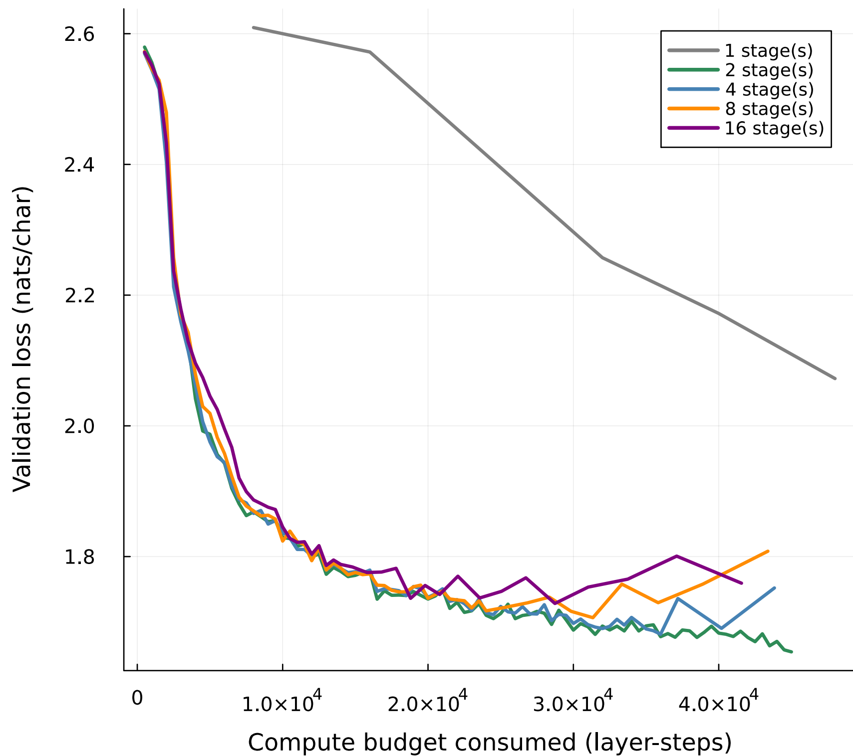
(a) Val loss vs. compute budget (1/L-weighted, mean of 2 seeds)
