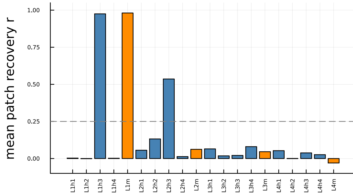
seed 33
