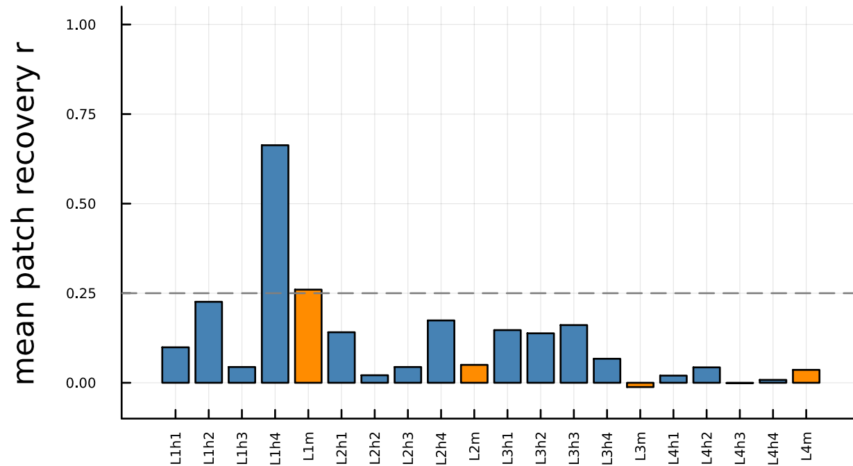
seed 11
