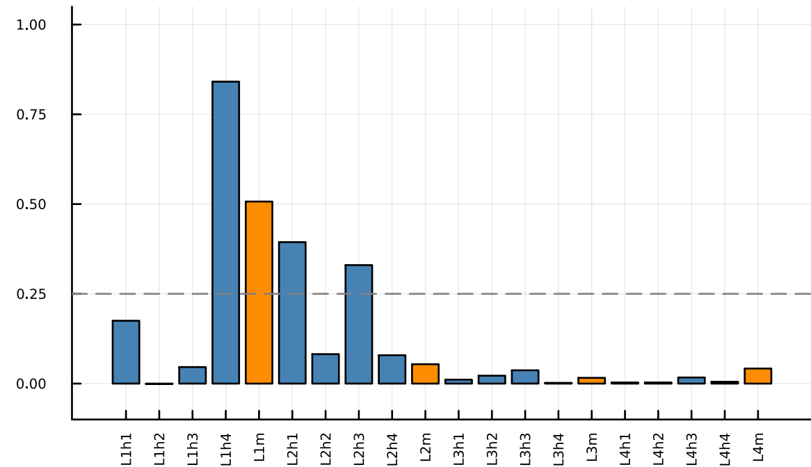
seed 22
