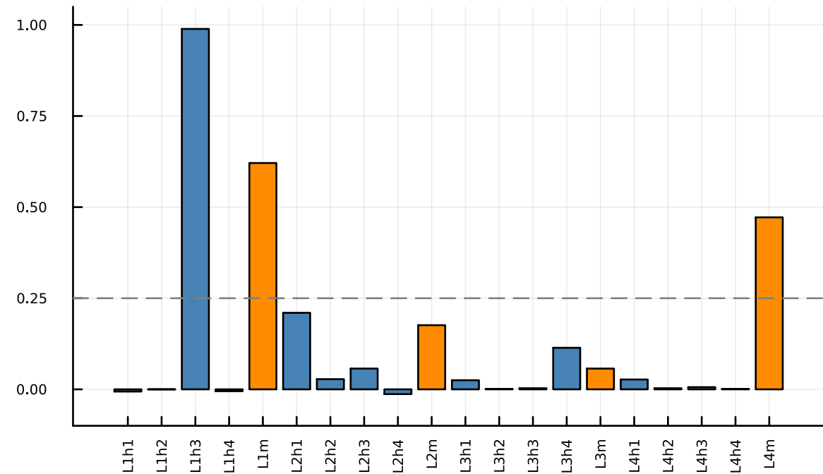
seed 44
