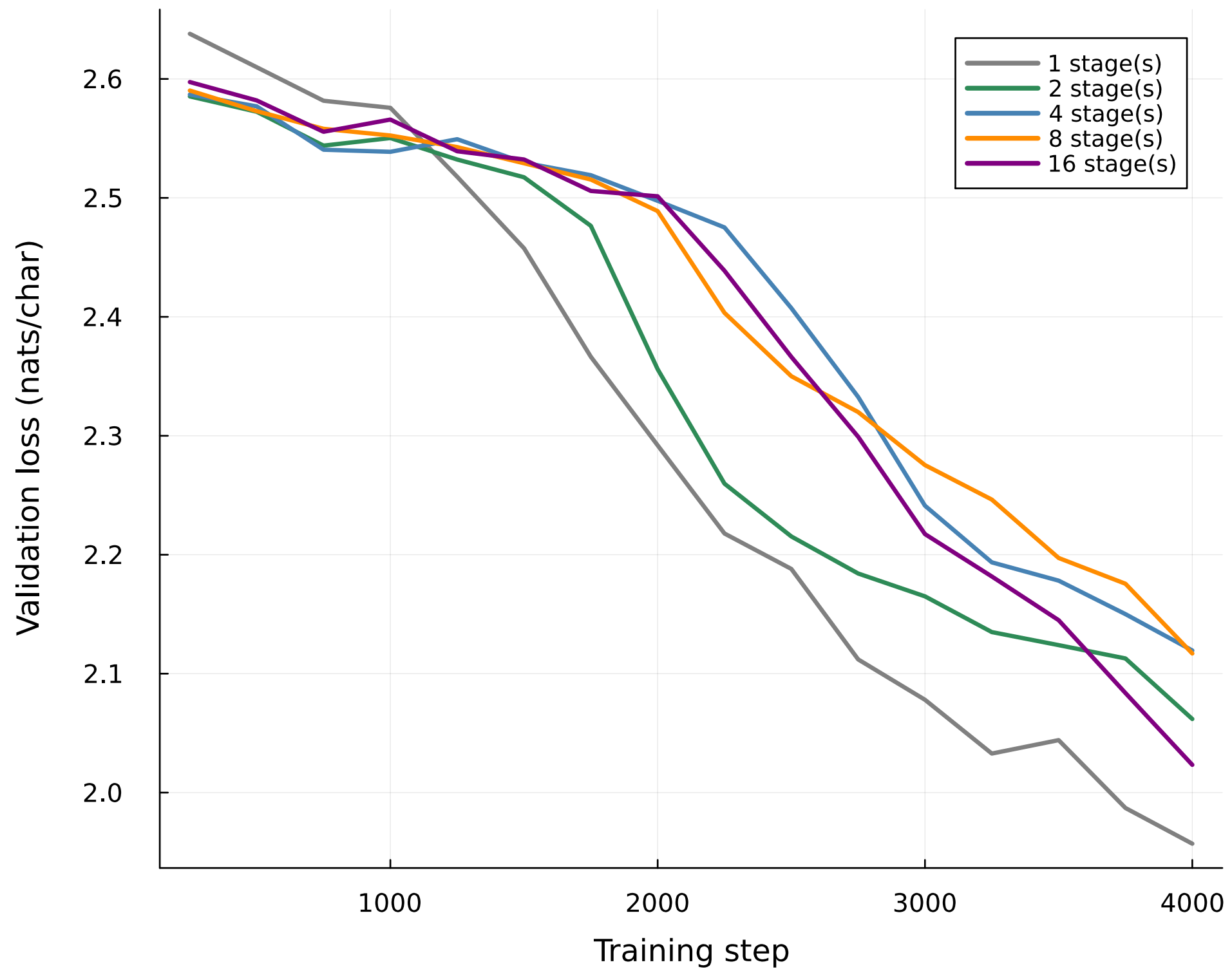
(a) Val loss vs. step (equal step count = 4000, mean of 2 seeds)
