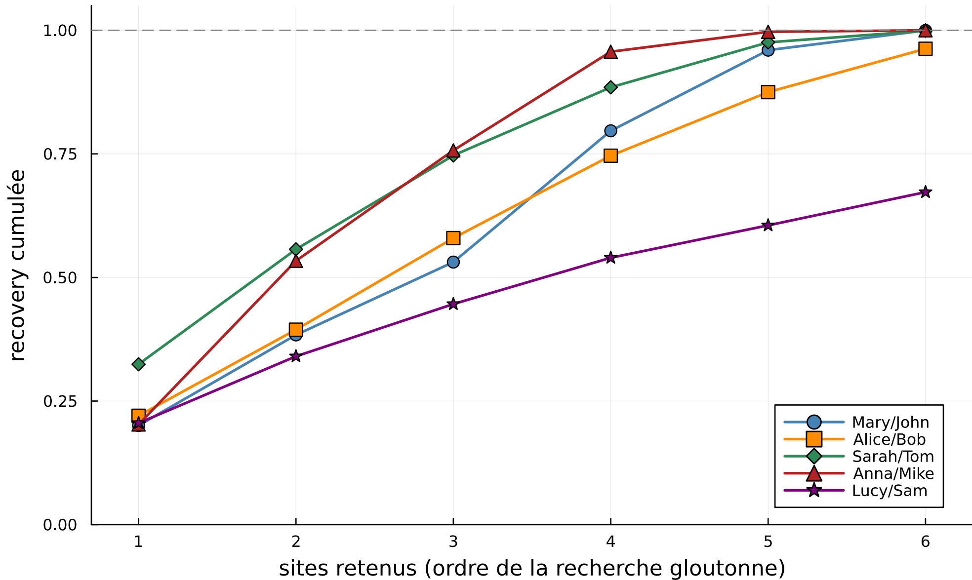
Recovery cumulée (greedy_patch_search!, max 6 sites), 5 instances IOI
