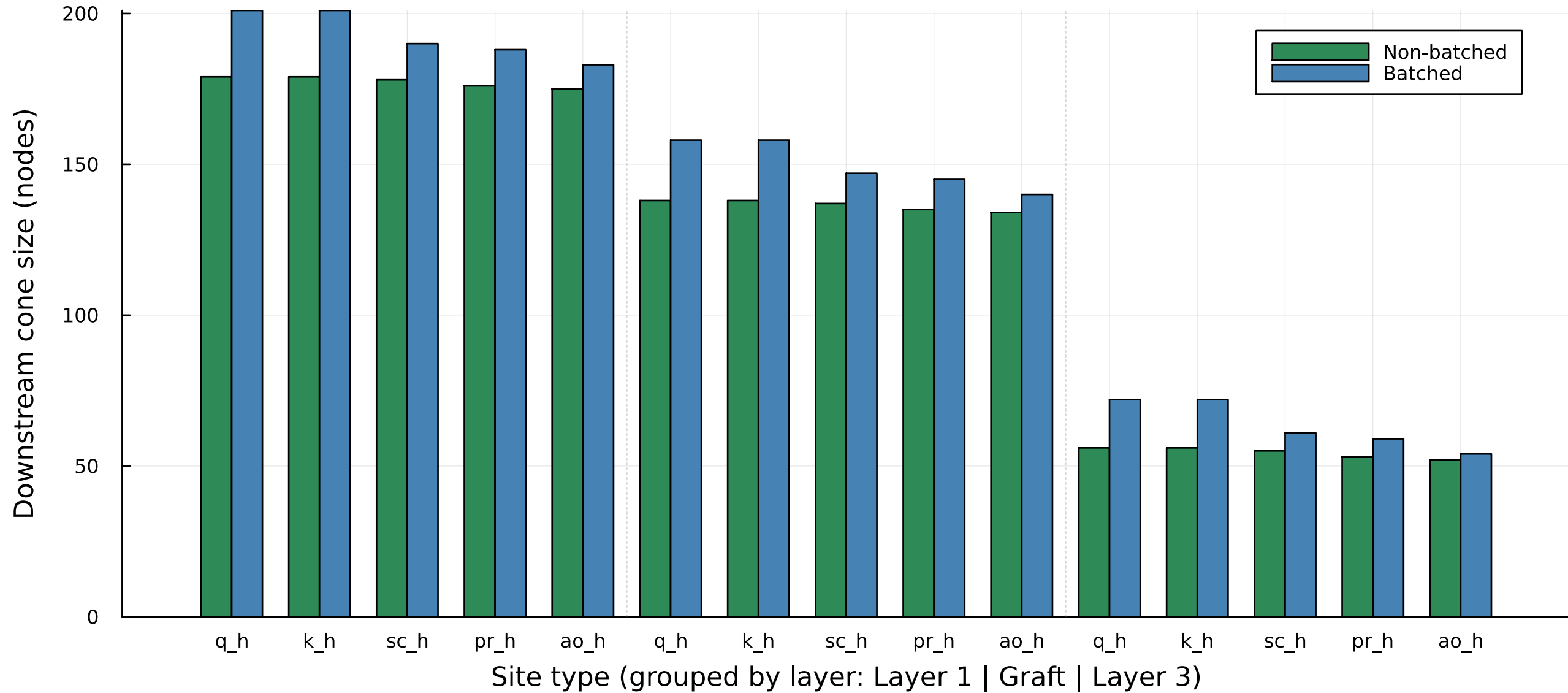
Patch cone size: batched vs. non-batched attention
