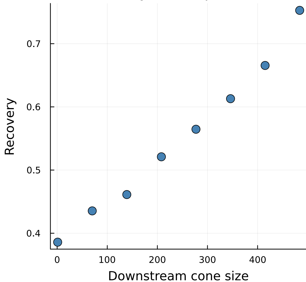
Across layers (depth varies)
