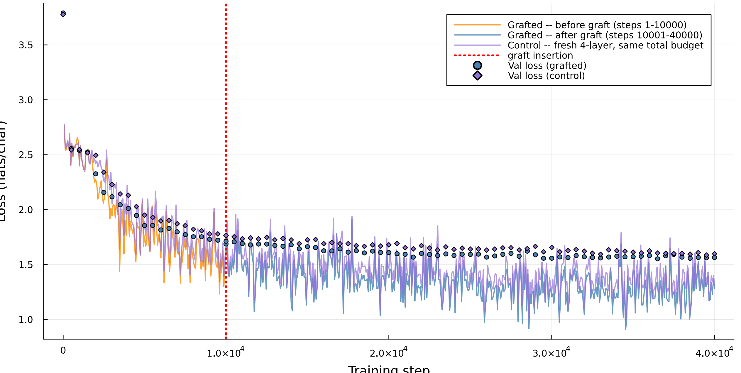
Hot surgery on a trained char-LM: grafted vs. equal-budget control
