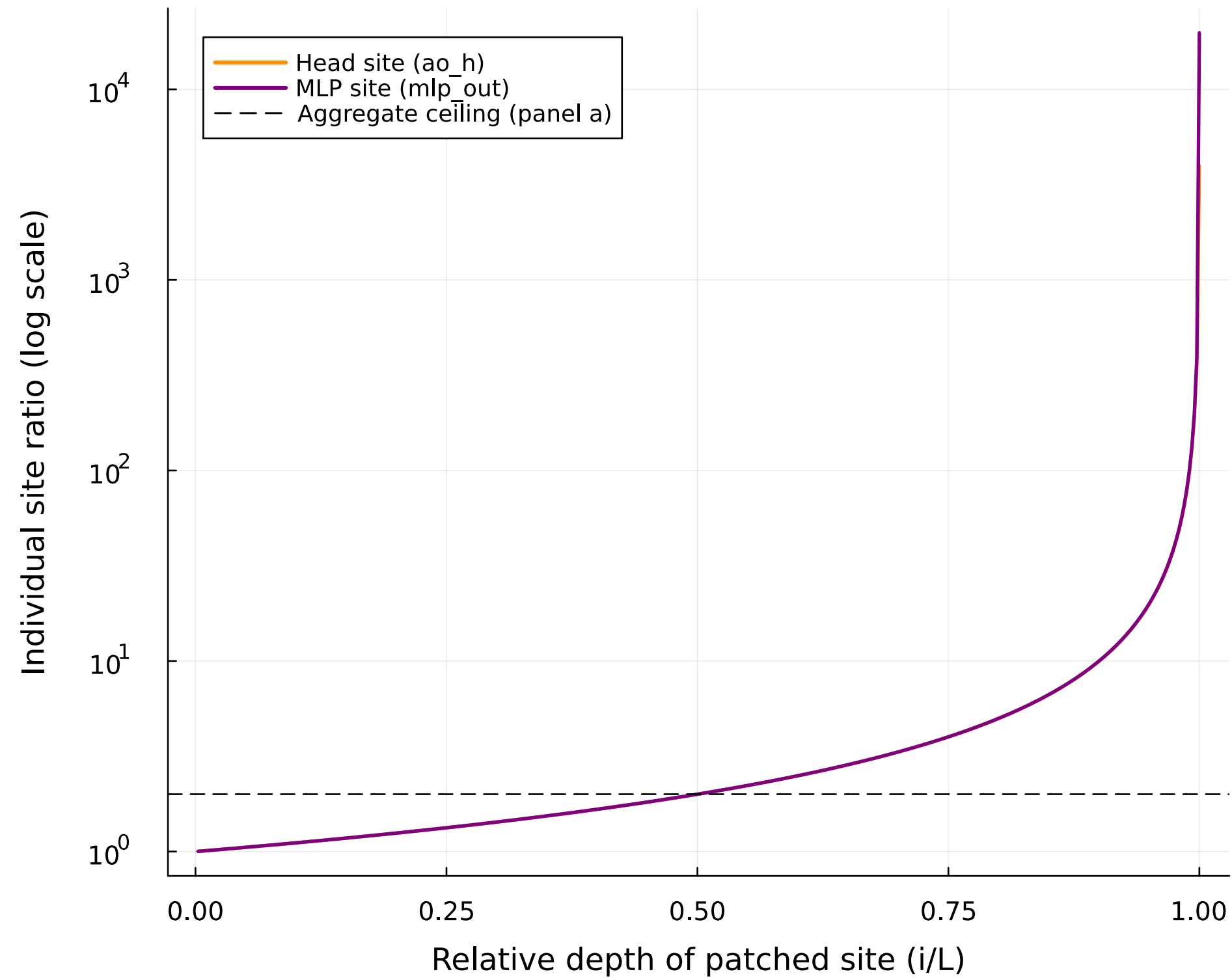
(b) Deep sites: individual ratio diverges
