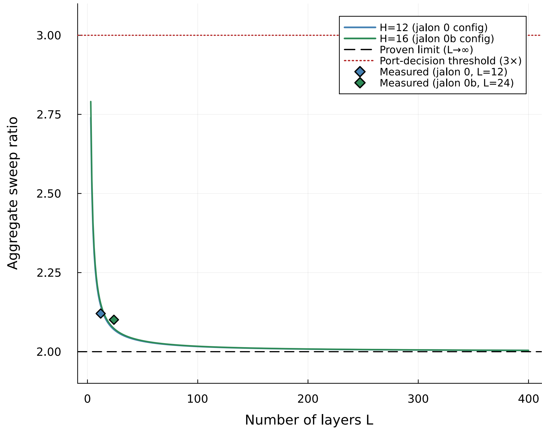
(a) Aggregate ratio \rightarrow 2 as depth grows
