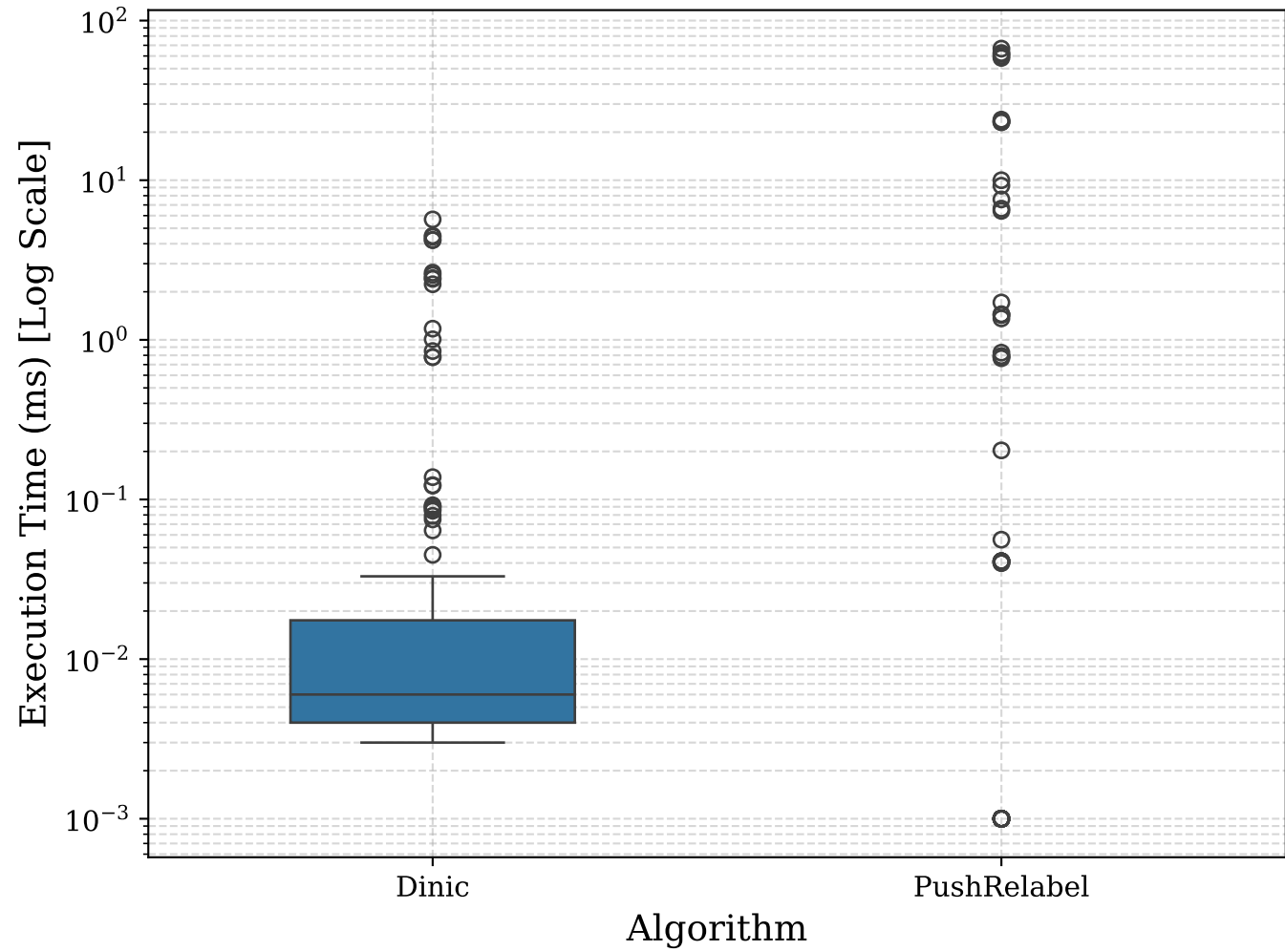
Execution Time Distribution across 50 Source-Sink Pairs
