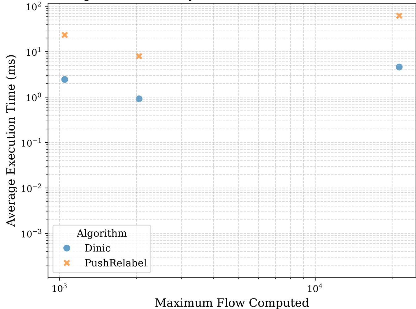
Algorithm Scalability: Execution Time vs. Flow Volume
