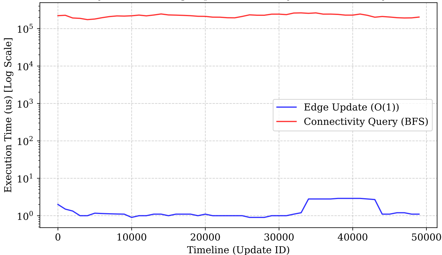
Dynamic Routing: Update vs. Query Time Scalability
