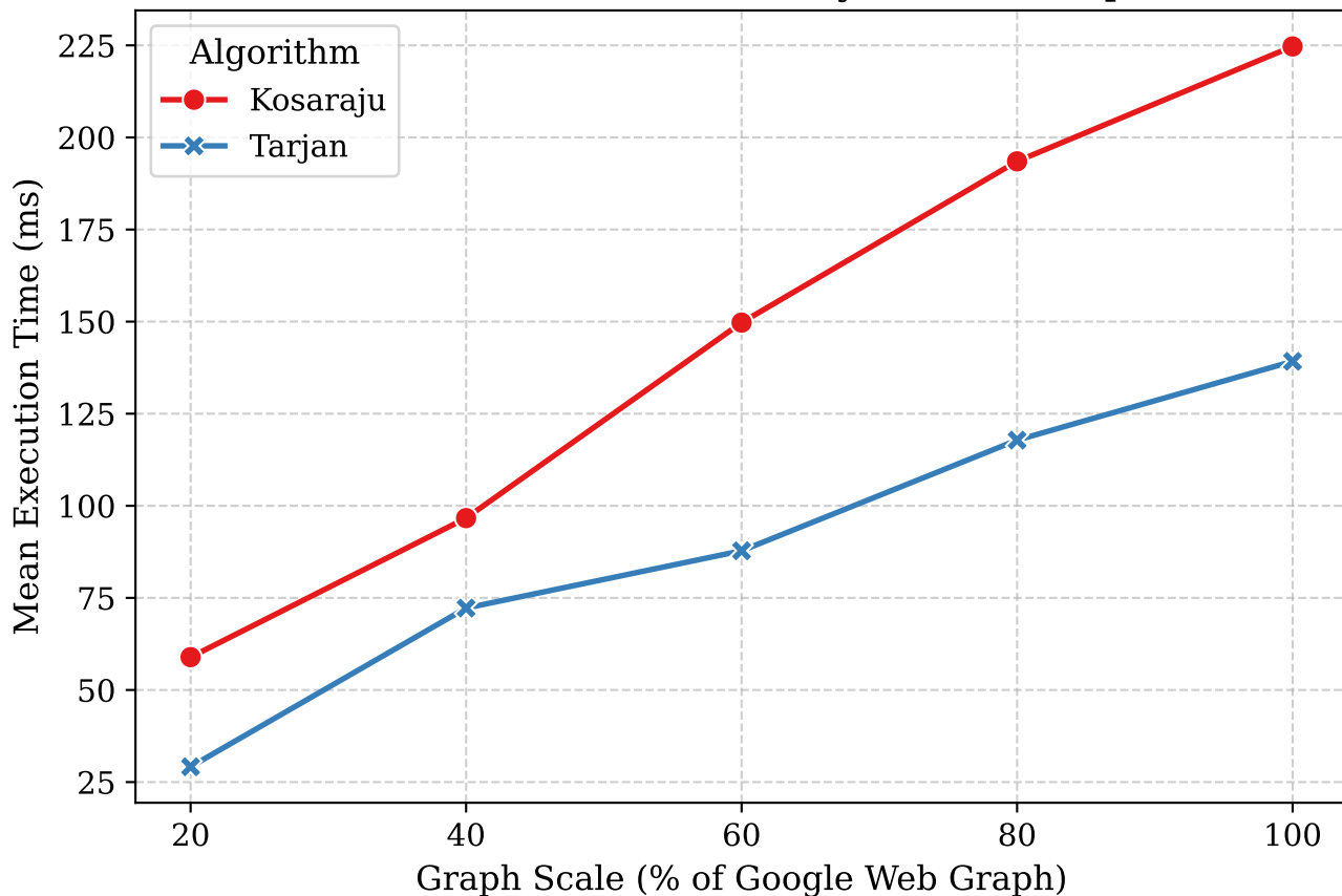
Execution Time Scalability on Web Graph
