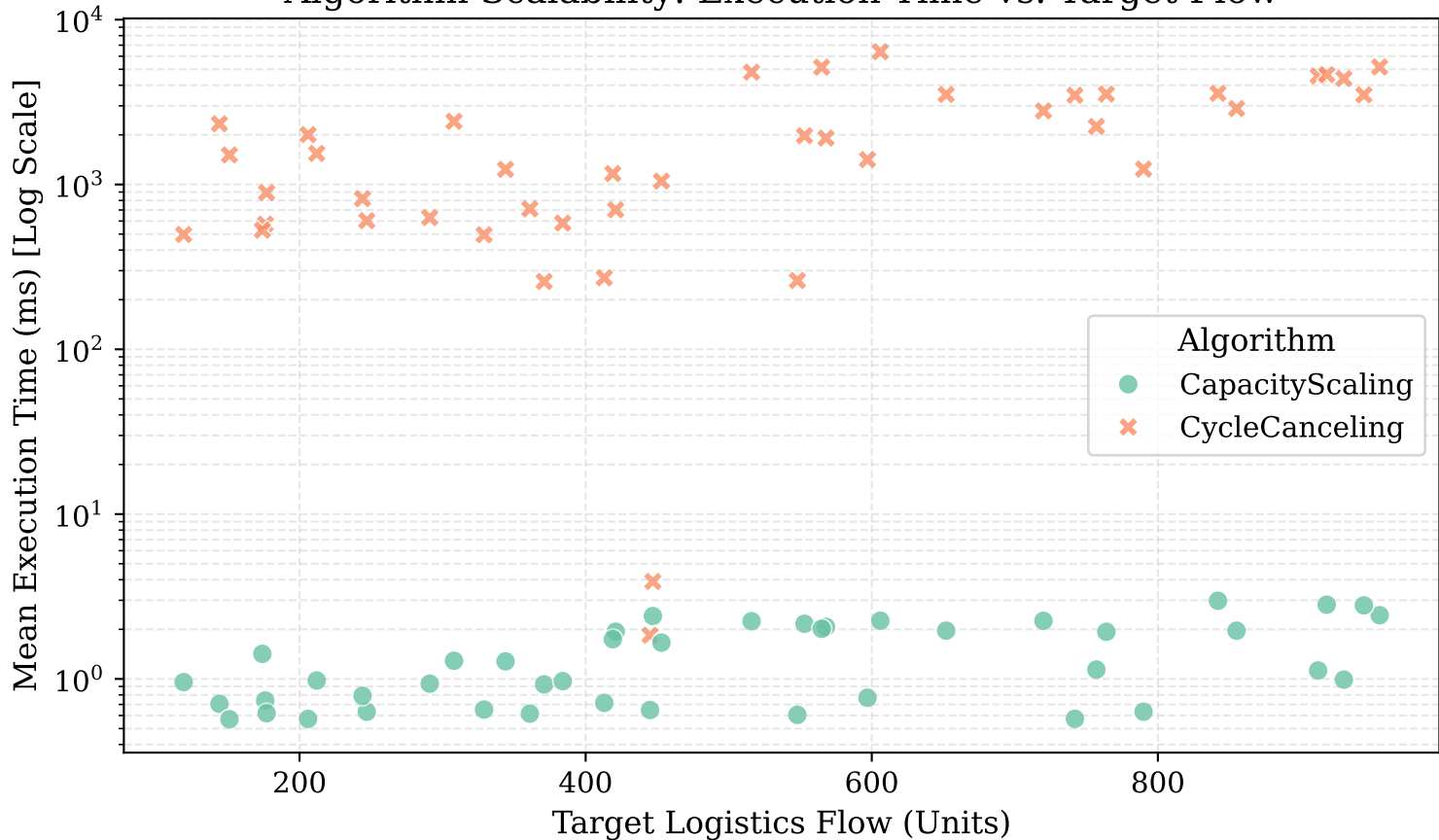
Algorithm Scalability: Execution Time vs. Target Flow
