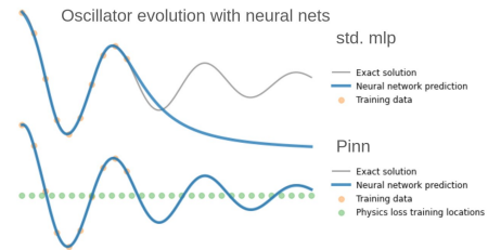
Figure 1: Example of the Pinn behavior.
