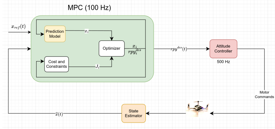
Figure 1: MPC control scheme for the quadrotor
