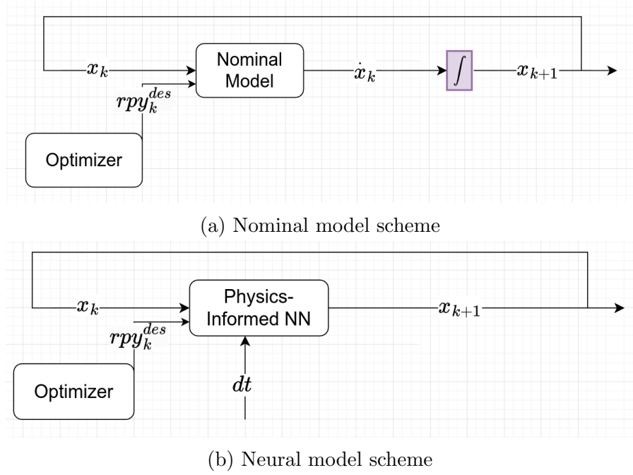
Figure 2: Comparison between traditional and neural model schemes
