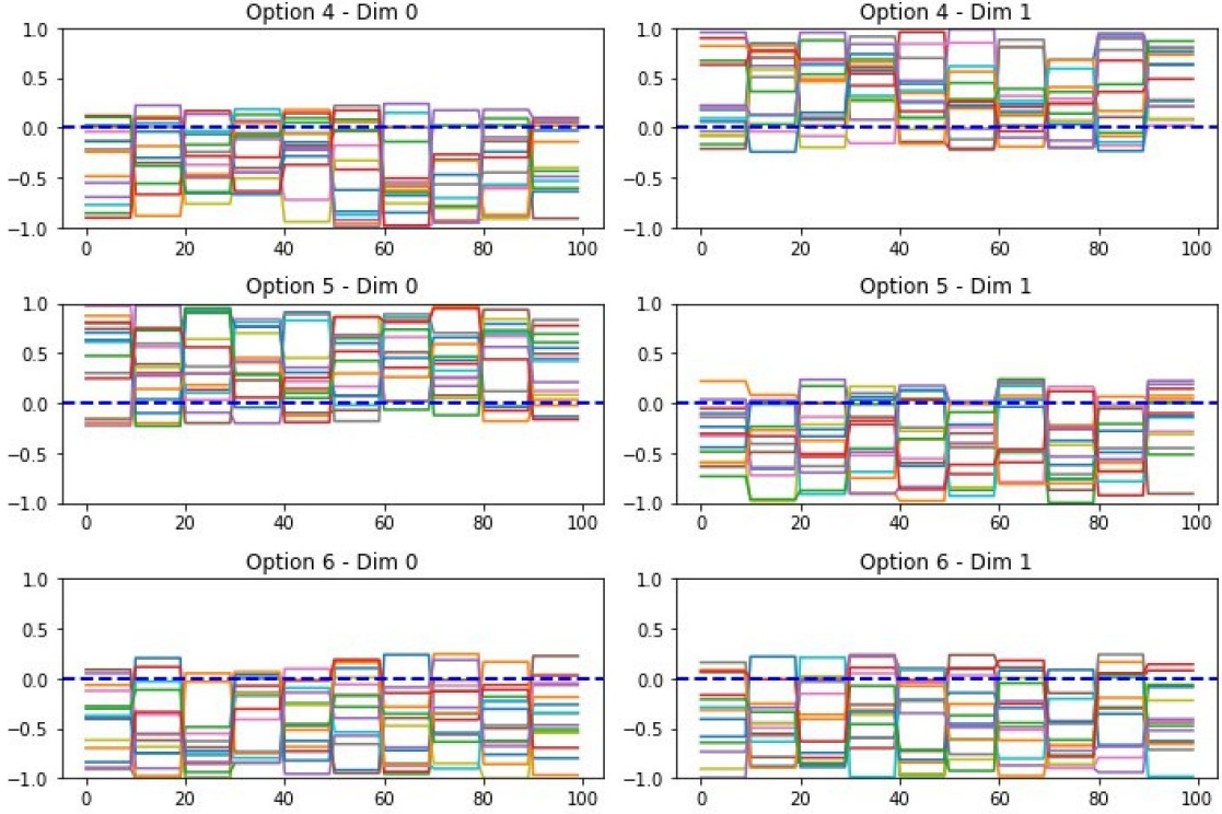
Figure 3: Example of the generated data for the unicycle (PiNN)
