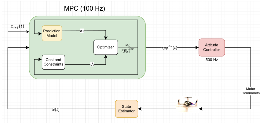
Figure: MPC control scheme for the quadrotor
