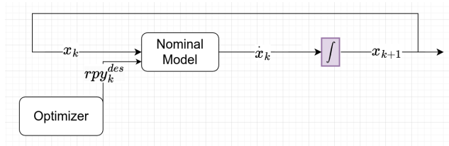
(a) Nominal model scheme
