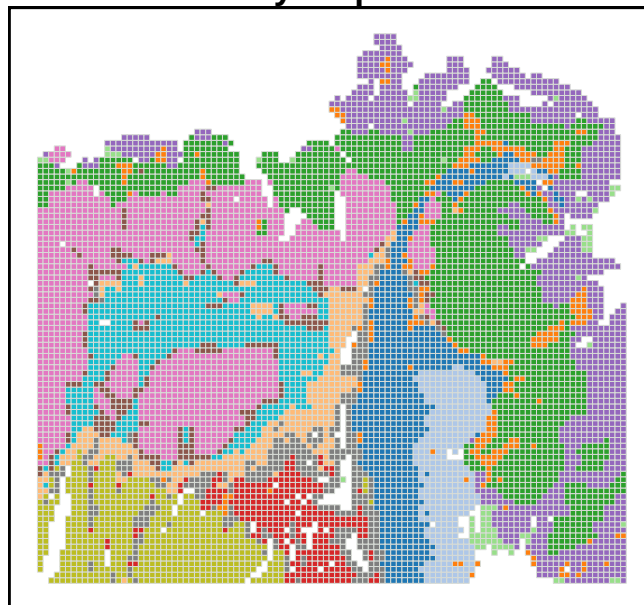
BayesSpace
