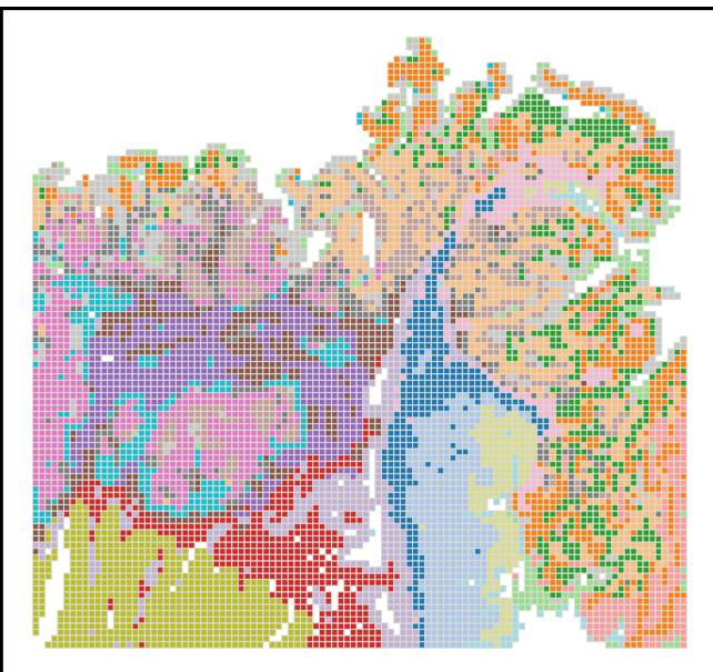
SCMEB
