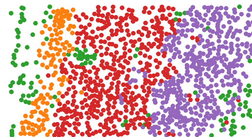
BANKSY: ARI=0.684
