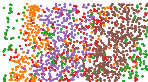
BASS: ARI=0.782
