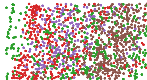
STAGATE: ARI=0.658
