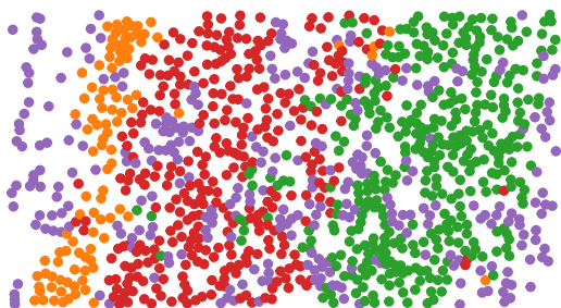
GraphST: ARI=0.414
