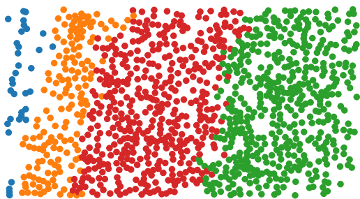
SCMEB: ARI=0.223
