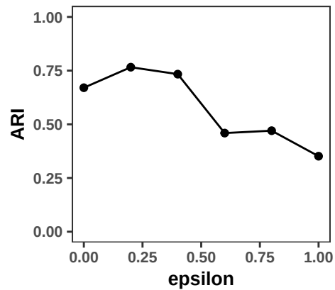
151672
