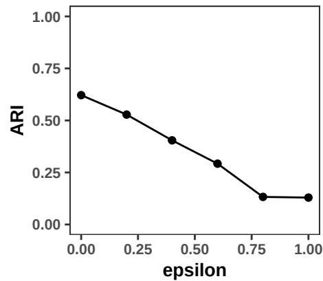
151671
