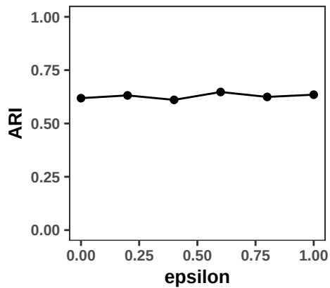
151670
