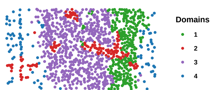
STAGATE: ARI=0.472
