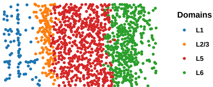
SCMEB: ARI=0.21
