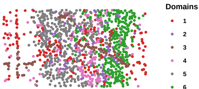
SCMEB: ARI=0.21
