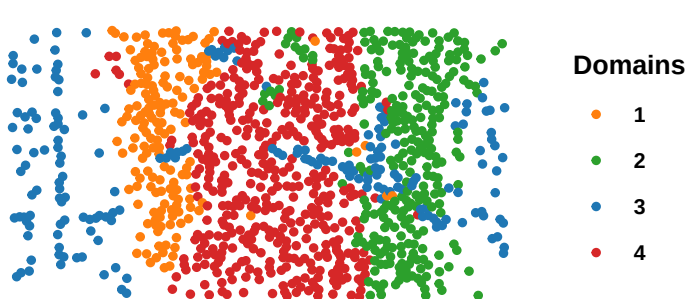
BASS: ARI=0.564
