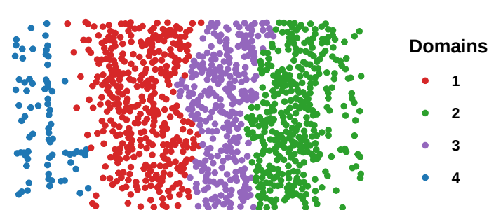
BANKSY: ARI=0.533
