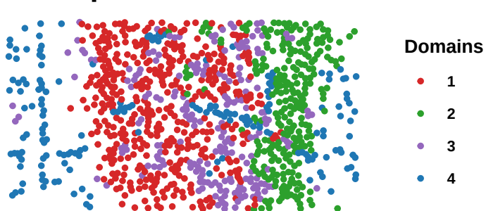
GraphST: ARI=0.327
