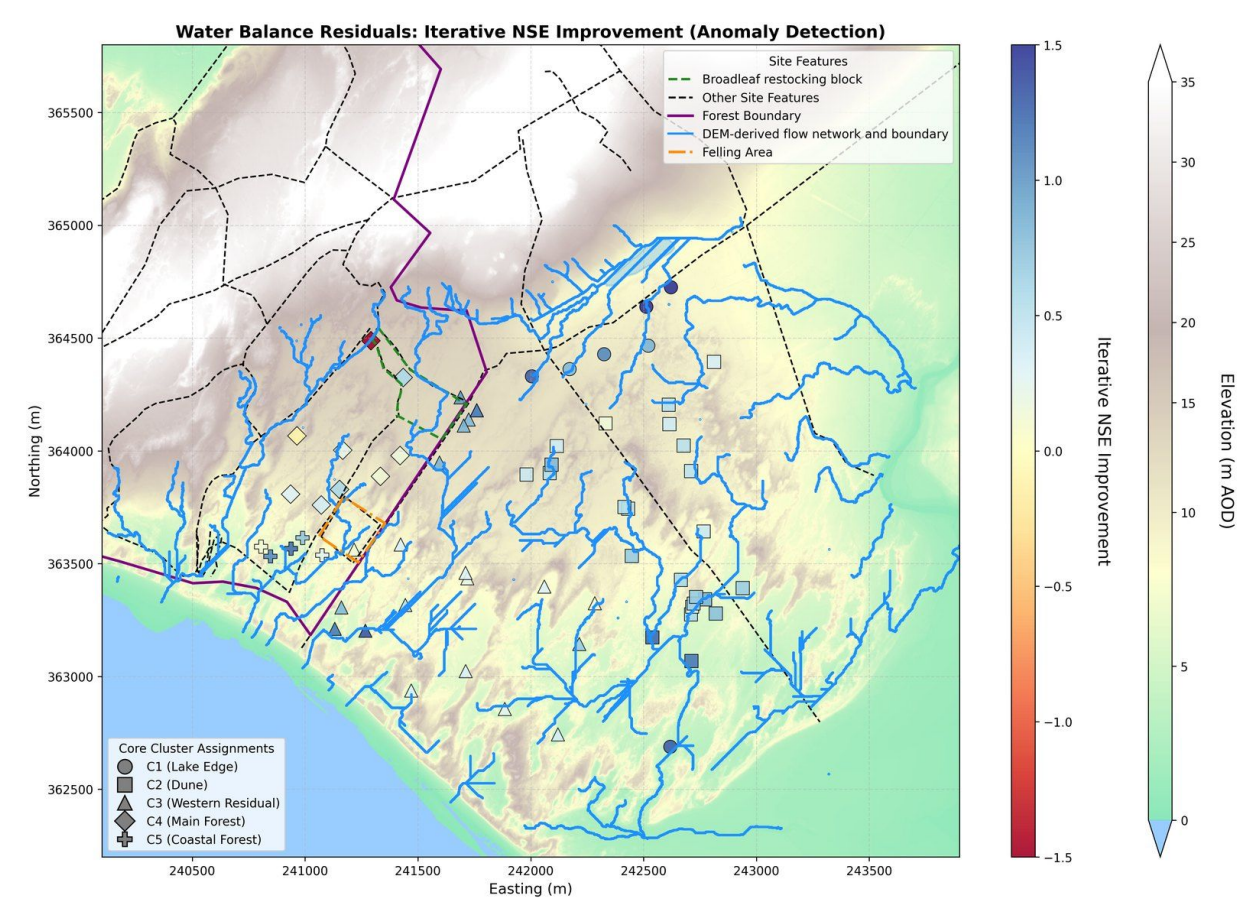
Figure 9. Spatial pattern of the SSM-over-TLM iterative Nash-Sutcliffe improvement across the reference network.
