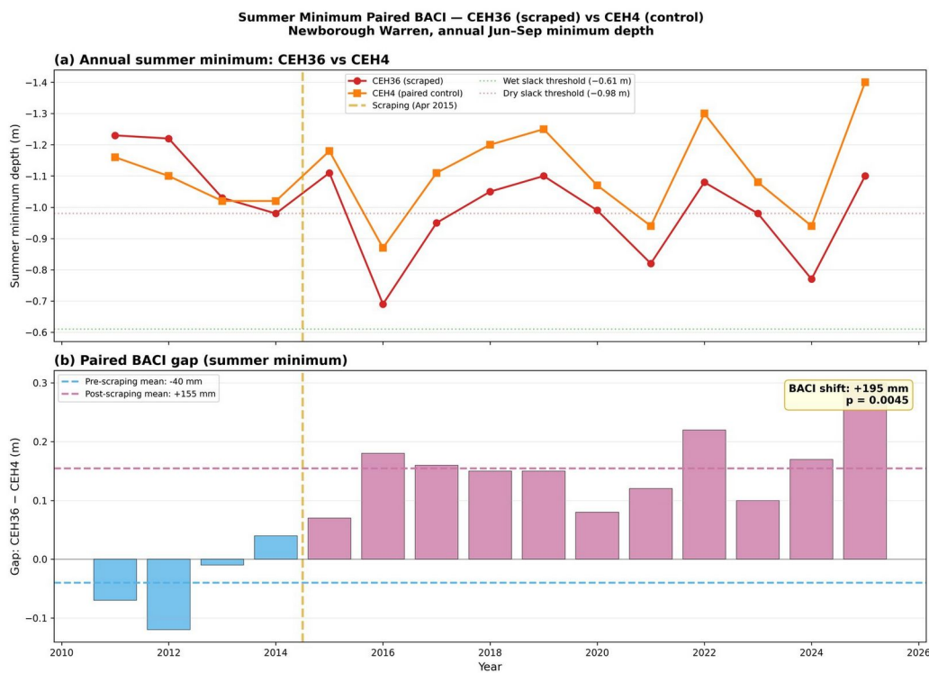
Figure 2. Paired BACI summer-minimum analysis, CEH36 (scraped) versus CEH4 (control) (measured). (a) Annual summer minimum depth with the Curreli et al. (2013) ecological thresholds. (b) BACI gap (CEH36 minus CEH4) by year, pre- and post-scraping means; the paired shift is +0.195 m ( p = 0.004 ). Source: 09c_04_summer_minima_paired.
