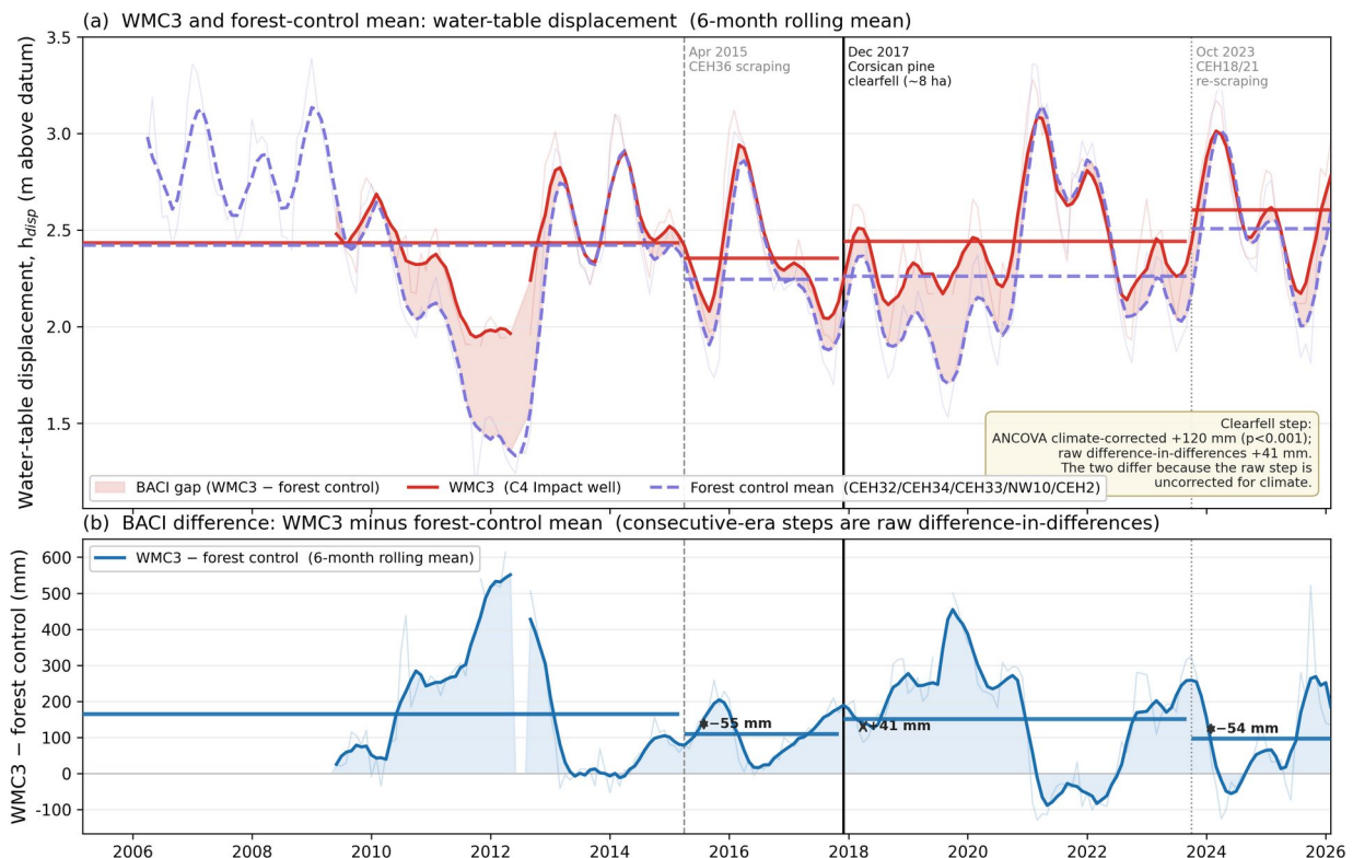
Figure 4. The felled well (WMC3, red) against the unfelled forest average (purple dashed), water levels relative to a fixed datum; shaded band is the gap between them. The gap widens after the December 2017 clearfell (+120 mm) and steps down at each scraping event (-55 mm in 2015, -54 mm in 2023) as the scrape draws the neighbouring water table down. Source: 10m_02_wmc3_baci_dual.png.
