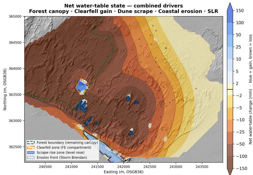
Figure 5. Parametric net water-table state: superposition of five annual-mean drivers — forest-canopy drawdown (edge deficit H_0 = 150 mm, removed within the clearfell footprint), dune-scrape contribution ( H_0 per cut; CEH36/18/21 measured, others assumed = CEH36), coastal erosion ( h_0 = 21 mm) and sea-level rise (+20 mm over 5 yr). All fields use a Euclidean-distance exponential-decay model. Symmetric \pm 150 mm diverging scale; bold zero contour. Source: 20_net_state_map.png.
