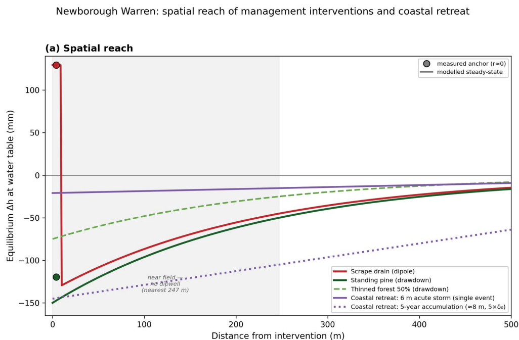
Figure 8. Spatial reach of management interventions and coastal retreat. Equilibrium head change as a function of distance from each source. Scrape benefit and forest drawdown decay exponentially (length scale \approx 225 m); coastal-retreat drawdown decays linearly to \approx 900 m. The two coastal curves differ in construction: the 6 m curve is a single storm-class event; the 5-year curve is five years' accumulation of the fitted retreat trend. All curves are modelled steady-state constructions anchored at two measured points (scrape BACI response; clearfell recovery). Source: 09f_management_effects.png.
