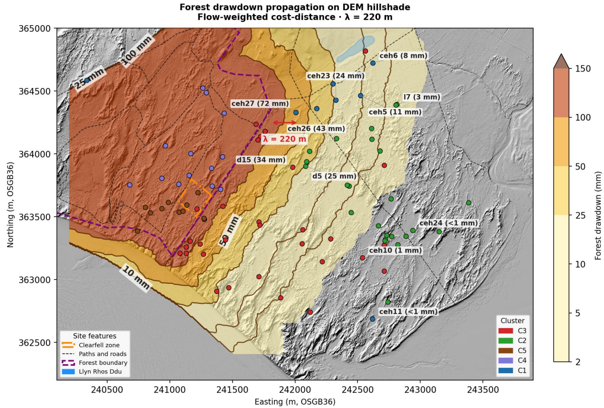
Figure 18. Illustrative forest reach. Forest-interception drawdown propagated inland from the plantation boundary by flow-weighted cost-distance (decay length \lambda \approx 220 m, from C3's specific yield and drainage coefficient combined with an assumed hydraulic diffusivity — a literature conductivity, K = 6 m/day (Betson et al., 2002), and a nominal 5 m saturated thickness, the latter poorly constrained and plausibly larger; assumed edge deficit). The reach is a scaling estimate rather than a calibrated length: across the range reported for dune sand ( K = 2 –20 m/day) \lambda spans roughly 130–410 m, and across a 3–8 m saturated thickness 170–280 m, so it is stated here to the nearest tens of metres. The mapped pattern depends only on the reach being of order 200 m rather than of order 20 m or 2 km, which holds across that whole range, over the DEM hillshade with per-well drawdown values labelled. The C3 wells fall within the forest reach while the C2 wells lie largely beyond it — drawdown falls from tens of millimetres near the plantation to under 1 mm at the easternmost C2 wells; the forest boundary, clearfell zone and Llyn Rhos-Ddu are marked. Drawdown magnitudes are illustrative of the reach rather than measured values; because the model represents canopy interception alone, its heads are a lower bound on the magnitude of the forest effect, and \lambda an upper bound on how far beyond the canopy that effect reaches.
