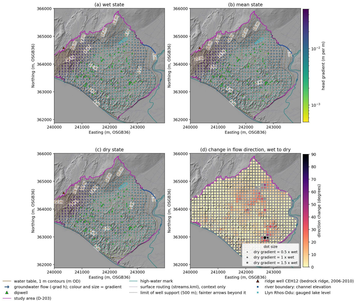
Figure 15. The water table kriged from the dipwells in (a) the wet state (wettest tenth of months), (b) the mean state and (c) the dry state (driest tenth), with 1 m contours (m OD). Arrows show the negative head gradient, one per 100 m square, sized and coloured by the gradient; arrows more than 500 m from a dipwell are faint, because there the boundaries rather than the wells set them. (d) The change in flow direction from wet to dry. Background: LiDAR hillshade (© NRW & OS).
