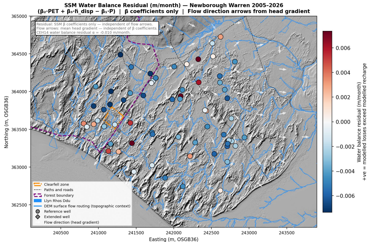
Figure 16. SSM water-balance residual at the 66 reference wells. Positive (red) indicates modelled losses exceeding modelled recharge; negative (blue) indicates over-prediction. The residual closes tightly across the network, with a small systematic negative offset: 65 of 66 reference wells lie within \pm 0.01 m/month and 51 are negative. No well exceeds +0.02 m/month; the largest positive value is NW3 (+0.0080 m/month). Rainfall is gross, and climate means are taken over the same period as the mean heads. Residuals are shown at the wells alone: no interpolation between wells predicts a withheld well's residual appreciably better than the network mean, so no surface is drawn. The residual is a diagnostic of a lumped-parameter model, not the output of a calibrated continuous-flow simulation.
