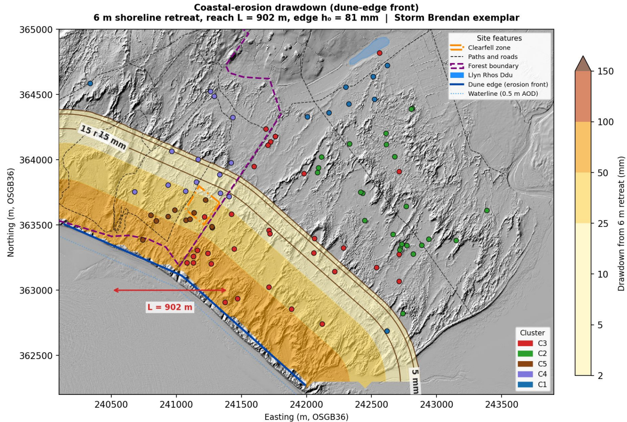
Figure 19. Episodic coastal-retreat reach. Water-table drawdown contoured inland from the eroding dune-edge front for a single Storm Brendan-scale retreat event ( \approx 6 m at the front, early 2020), over the fitted inland reach ( L_{cg} \approx 900 m; §4.11). Coastal retreat at this shore is episodic, concentrated in storm events; the per-event edge drawdown is scaled from the chronic gradient through the retreat rate measured over the same period as that gradient ( E_c = 2.32 m/yr, 2006–2026, from shoreline positions digitized in this study). The C3 wells fall within the reach while the C2 wells lie largely east of it; the forest boundary and Llyn Rhos-Ddu are marked.
