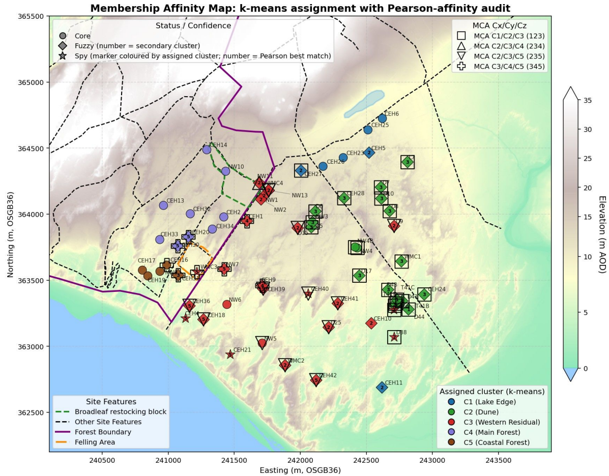
Figure 5. Spatial distribution of the five hydrogeological clusters (Pearson affinity validation), reference network (66 wells). Points coloured by k-means assignment; circles = Core ( \Delta r > 0.05 ), diamonds = Fuzzy ( \Delta r < 0.05 ; number inside diamond = secondary cluster), stars = Spy (Pearson best-match / assigned; number inside star = best-match cluster). Hollow overlays = Multi-Cluster Affinity ( r > 0.90 with \geq 3 clusters). LiDAR: © NRW & OS.
