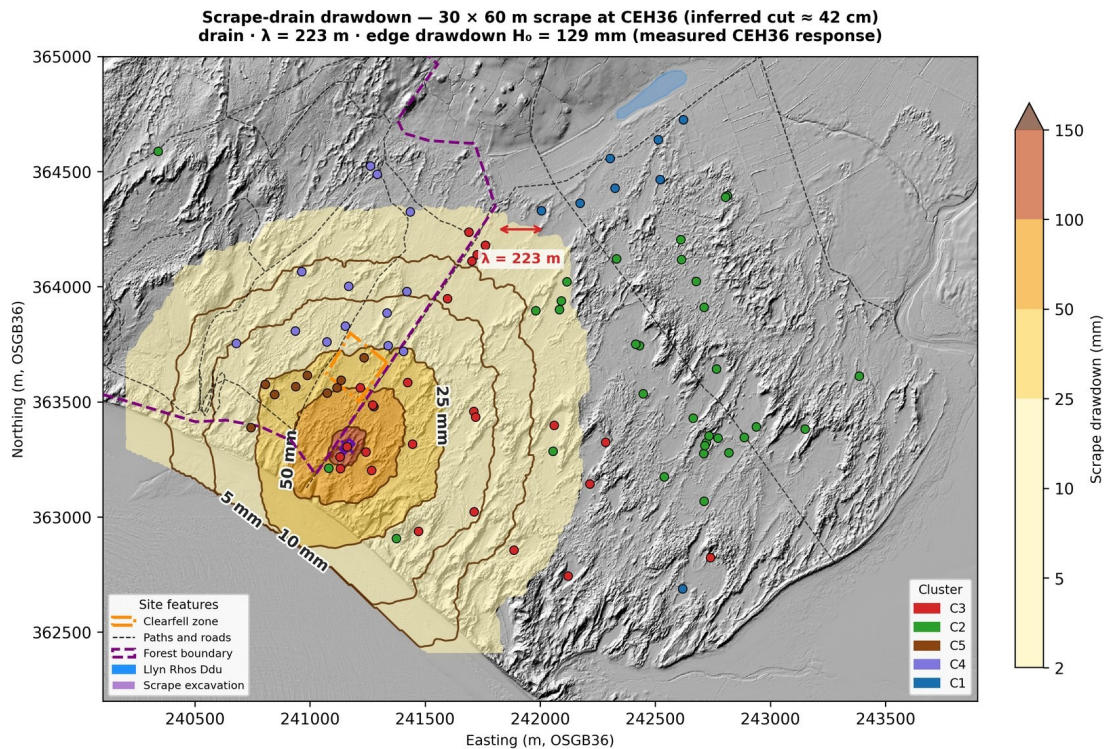
Figure 8. Modelled steady-state drawdown field around the 2015 CEH36 scrape — edge magnitude empirically anchored, reach modelled. The edge drawdown is set to the measured CEH36 scraping response (≈0.13 m; Script 09a, Pure-Scraping era vs CEH4), not an assumed value; the surrounding field is a steady-state radial-drain decay along a flow-weighted cost-distance (leaky-aquifer length \lambda = \sqrt{K \cdot b / (S_y \cdot \beta_3)} \approx 230 \text{ m} ), with the excavation interior masked because the slack itself rises. The excavation depth (≈0.42 m) is the inferred output, D = H_0 / S_y , not a survey input. The elevated displacement head at the scrape steepens drainage gradients and draws the surrounding water table down — the same mechanism as coastal erosion, underlying the chase-inland cascade. Source: 20_scrape_drawdown_nohead.
