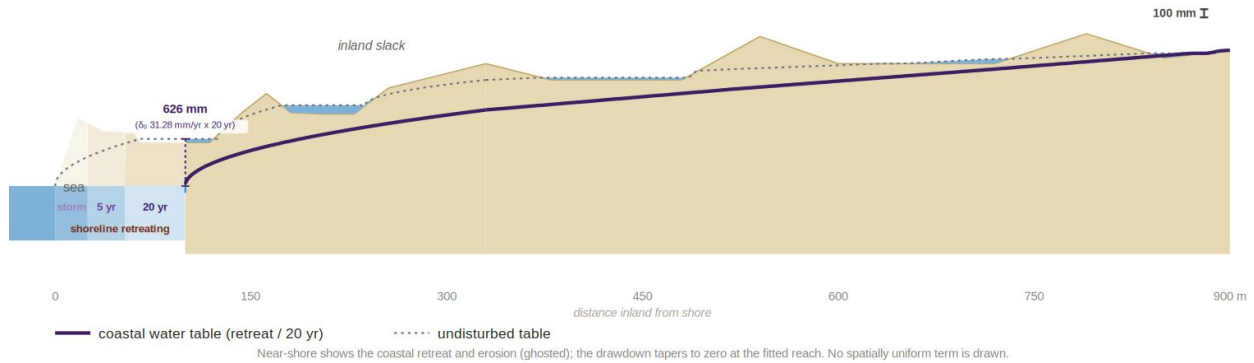
Figure 20. Conceptual reach of coastal retreat and the far-field term. Long-section from the eroding Caernarfon Bay shoreline inland to 900 m, drawn so that the fitted inland reach L_{cg} \approx 900 m (§4.11) falls at the right-hand edge; the dune surface and its slack are illustrative, the vertical scale is exaggerated \times 58 , and a 100 mm bar is given for reference. The coastal water table (solid) is the fitted coast-edge trend accumulated over a twenty-year horizon, declining linearly to zero at the fitted reach; the undisturbed table (dotted) is the same surface without it. At 150 m, where the headline rate is quoted, the twenty-year accumulation is 528 mm. The curve is drawn in to the shoreline, where the fitted amplitude \delta_0 = 31.28 mm/yr gives 626 mm; that value is an extrapolation beyond the nearest well, which sits at 147 m. The fitted far-field constant c_{far} ( -0.3 mm/yr, \approx -6 mm accumulated over the same horizon) is a window statistic rather than a rate (§4.11) and is not drawn: over this reach coastal retreat is the only identified distance-dependent term. The ghosted wedges at the shore mark the shoreline positions implied by a single 6 m storm event and by five- and twenty-year accumulations of the mean retreat rate. The section is a schematic built from the fitted parameters rather than a modelled water-table surface. Adapted from the technical report (Hollingham, 2026d).
