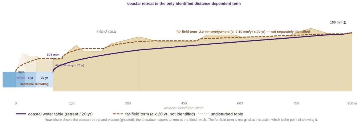
Figure 21. Conceptual reach of coastal retreat and the far-field term. Long-section from the eroding Caernarfon Bay shoreline inland to 900 m, drawn so that the fitted inland reach L_{cg} \approx 900 m (§4.11) falls at the right-hand edge; the dune surface and its slack are illustrative, the vertical scale is exaggerated \times 62 , and a 100 mm bar is given for reference. The coastal water table (solid) is the fitted coast-edge trend accumulated over a twenty-year horizon, declining linearly to zero at the fitted reach; the undisturbed table (dotted) is the same surface without it. At 150 m, where the headline rate is quoted, the twenty-year accumulation is 524 mm. The curve is drawn in to the shoreline, where the fitted amplitude \delta_0 = 31.35 mm/yr gives 627 mm; that value is an extrapolation beyond the nearest well, which sits at 147 m. The fitted far-field constant c_{far} ( -0.10 mm/yr, \approx -2.0 mm accumulated over the same horizon) is a window statistic rather than a rate (§4.11) and is not drawn: over this reach coastal retreat is the only identified distance-dependent term. The ghosted wedges at the shore mark the shoreline positions implied by a single 6 m storm event and by five- and twenty-year accumulations of the mean retreat rate. The section is a schematic built from the fitted parameters rather than a modelled water-table surface. Adapted from the technical report (Hollingham, 2026a).
