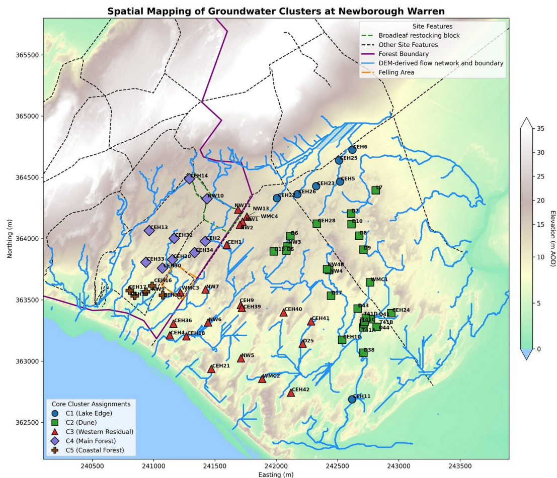
Figure 4. Spatial mapping of the five groundwater clusters identified by the analysis. Each colour represents a zone with distinct behaviour: C1 Lake Edge (blue), C2 Dune (green), C3 Western Residual (red), C4 Main Forest (purple), C5 Coastal Forest (brown).
