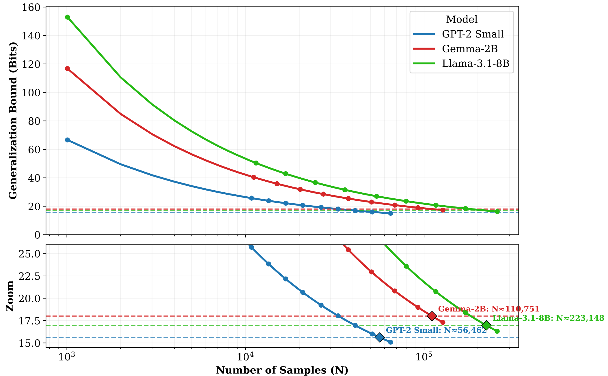
Sparse Semantic Generalization Bound (Concept Pool)
