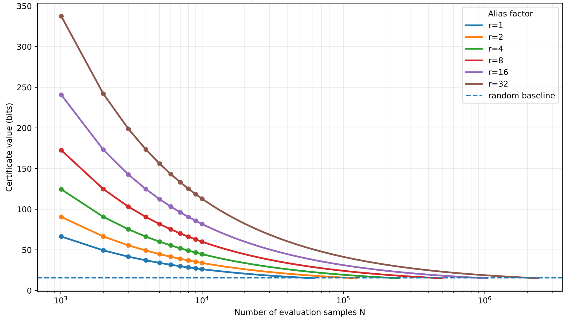
Feature-fragmentation control: GPT-2 Small
