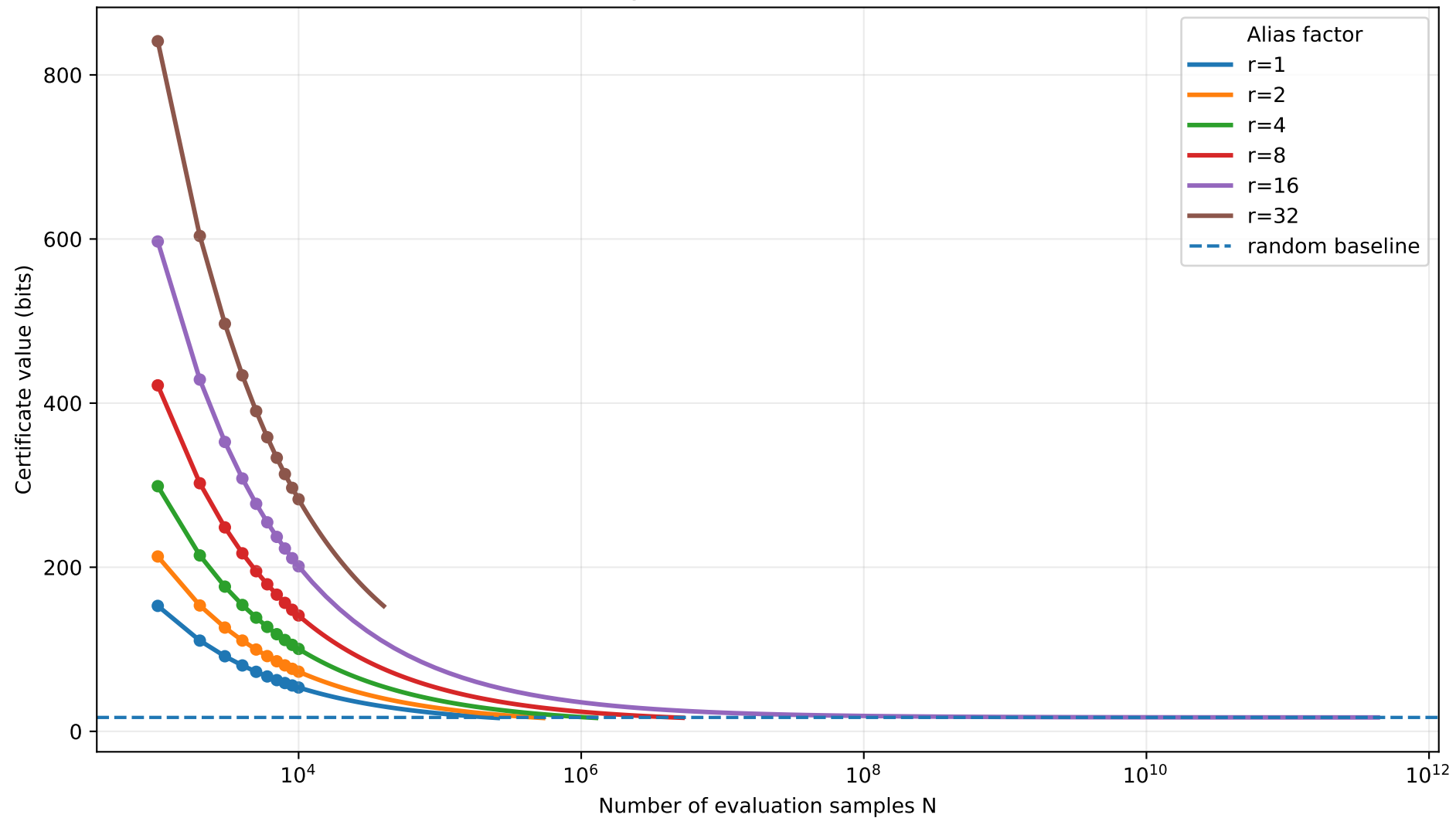
Feature-fragmentation control: Llama-3.1-8B
