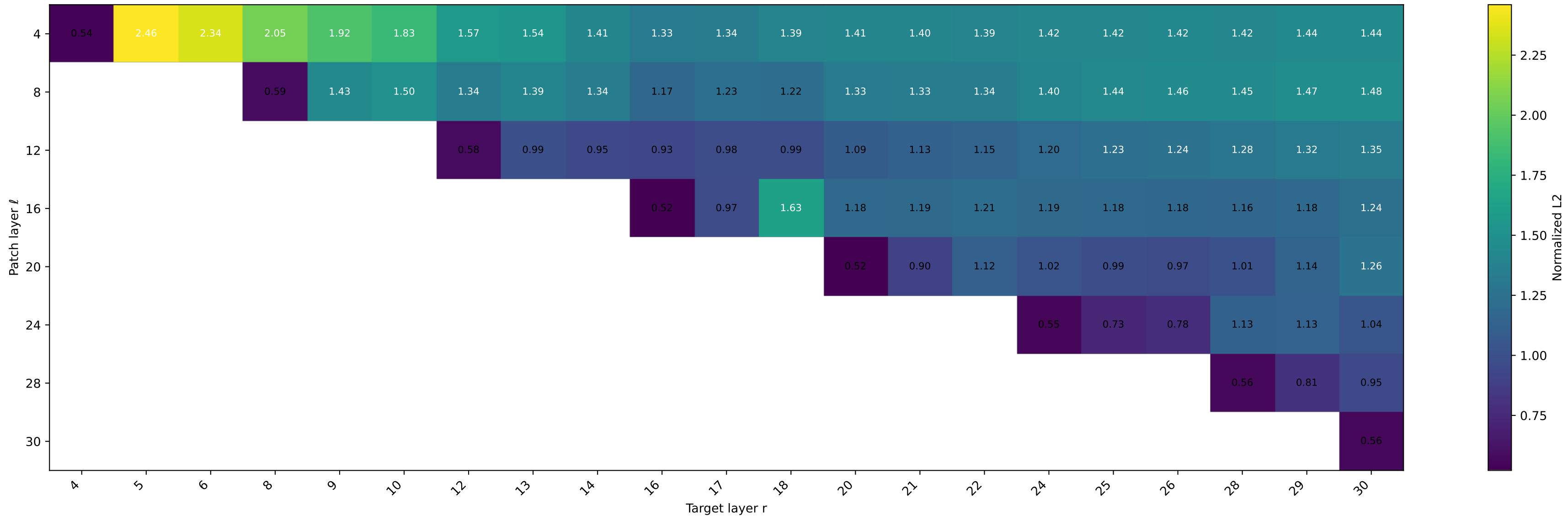
Llama-3.1-8B: SAE reconstruction (Normalized L2)
