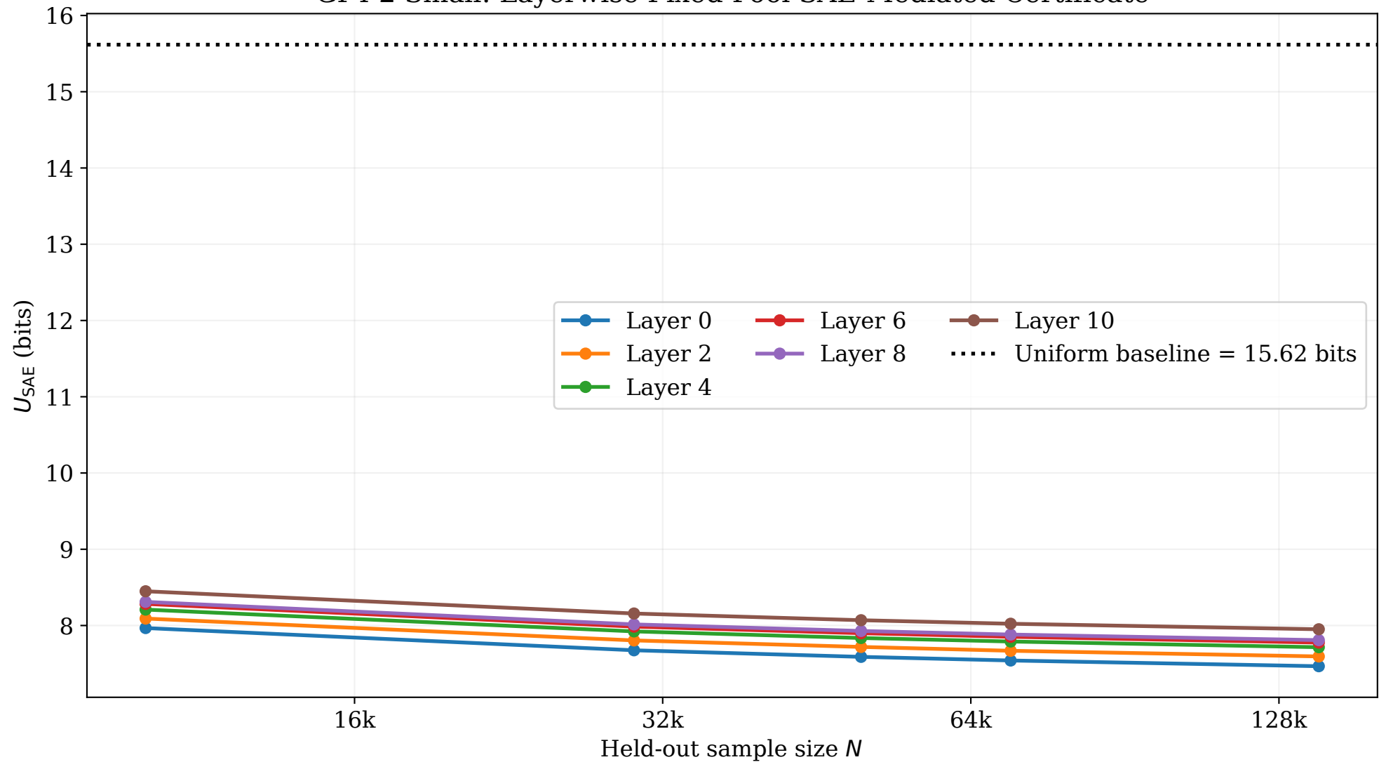
GPT-2 Small: Layerwise Fixed-Pool SAE-Mediated Certificate
