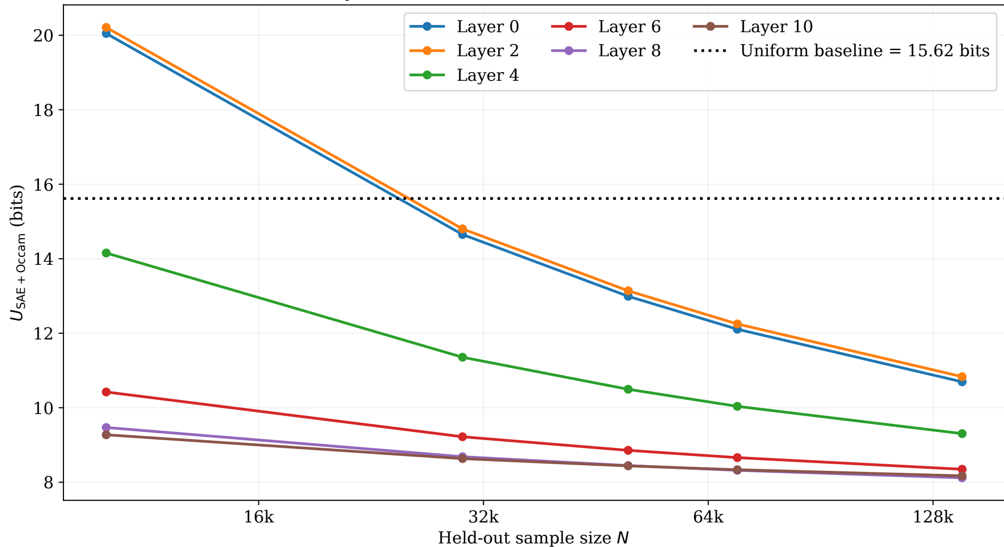
GPT-2 Small: Layerwise SAE-Mediated Certificate (Exact- \mathcal{P} Extension)
