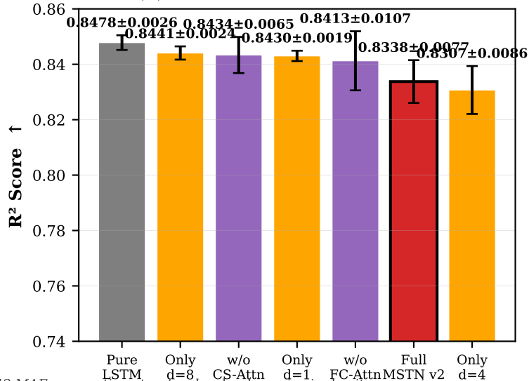
(b) R 2 across Ablation Variants
