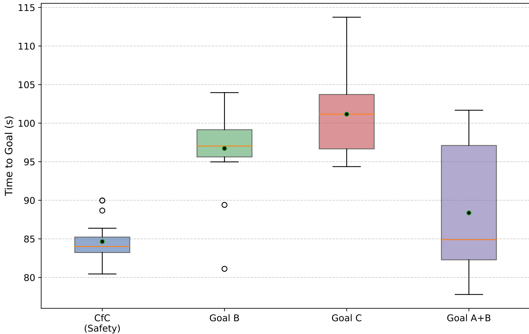
Time-to-Goal Distribution (Goal Generalization)
