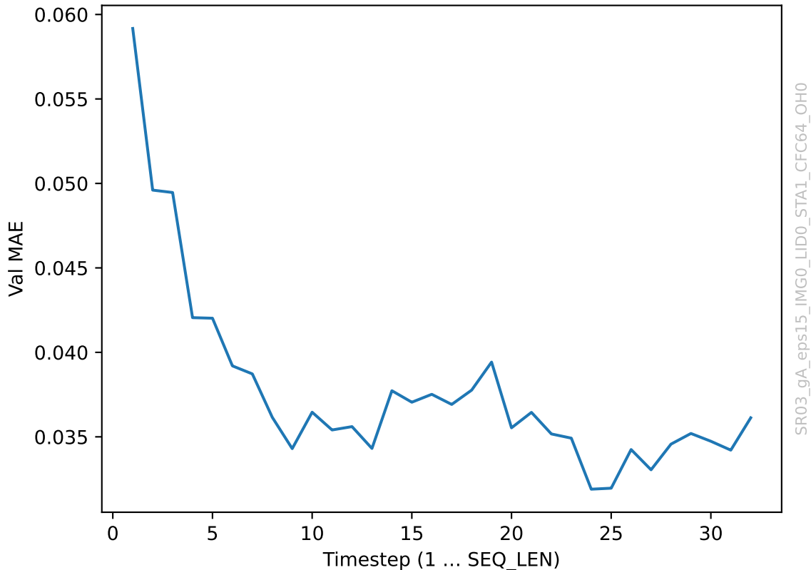
Per-timestep Validation MAE
