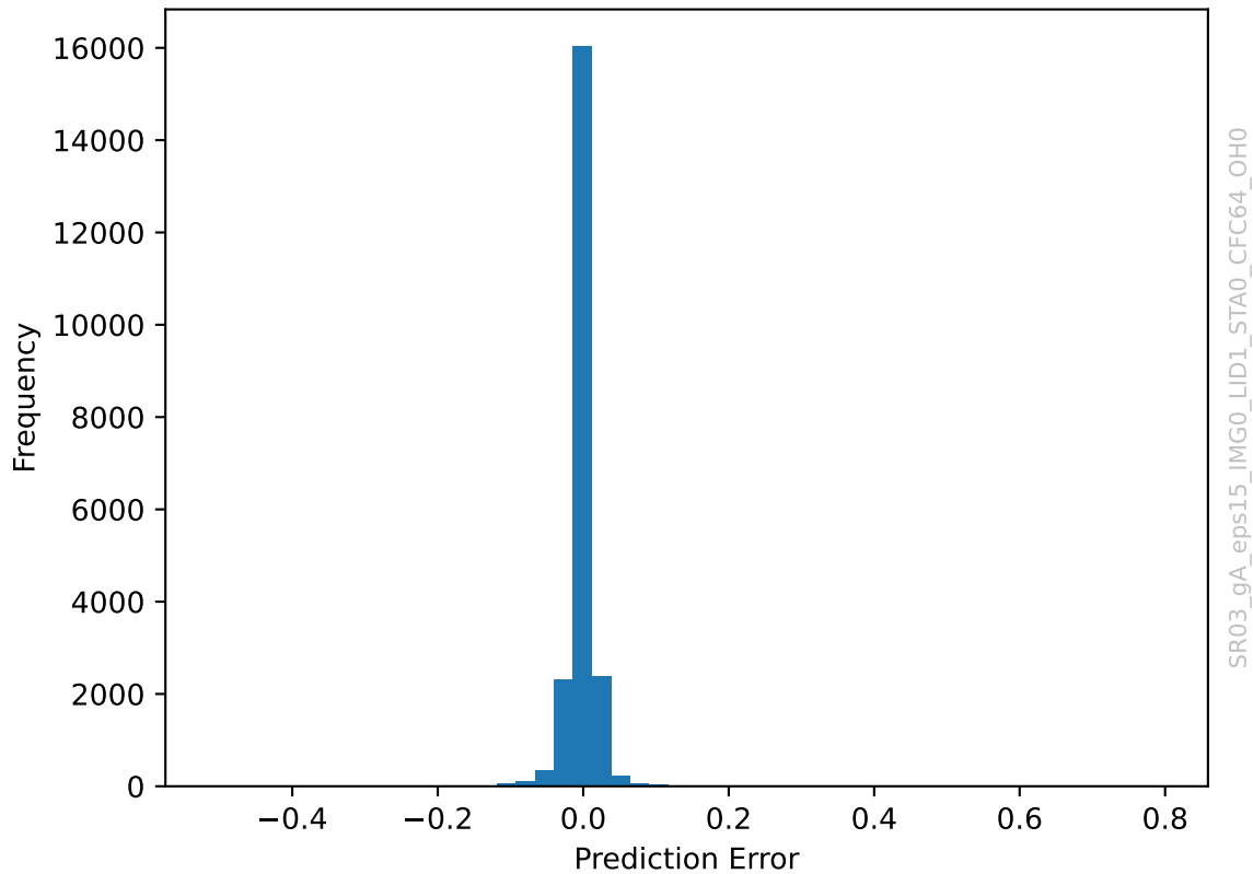
Linear Velocity Error Histogram
