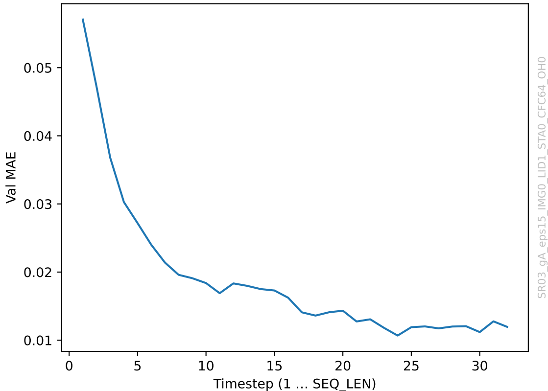
Per-timestep Validation MAE
