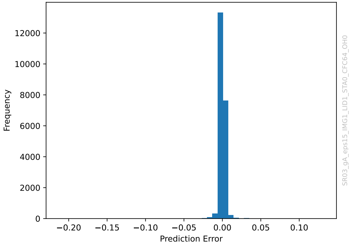
Angular Velocity Error Histogram
