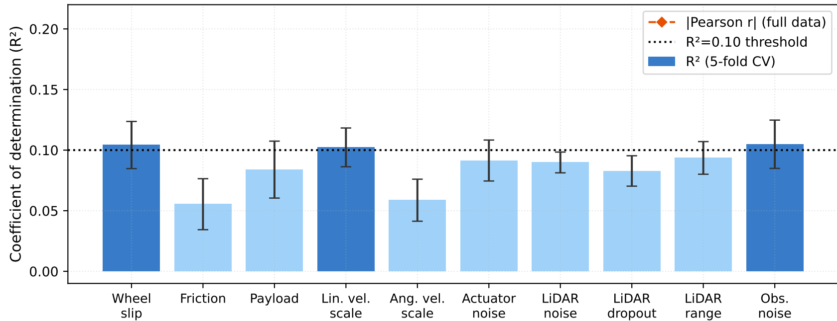
P4: Context Identifiability — linear probe from z to hidden dynamics params ( n=1500 episodes, 5 CADRE seeds)
