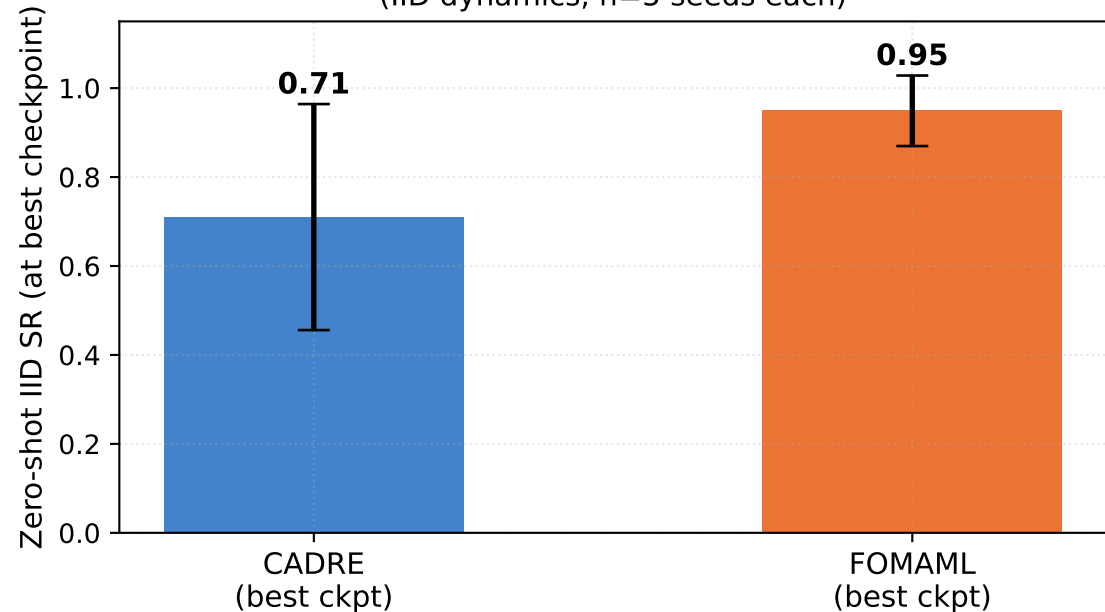
Zero-shot performance at best checkpoint (IID dynamics, n=5 seeds each)
