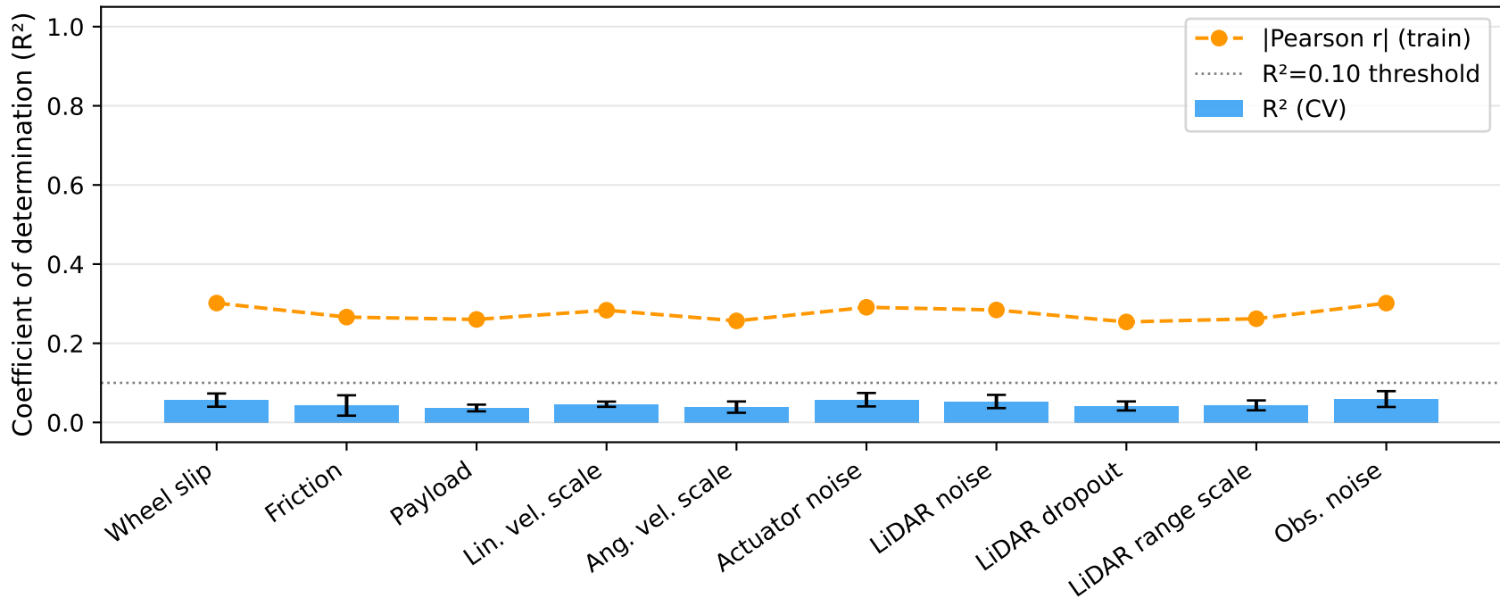
Context Identifiability (pooled across 5 seeds)
