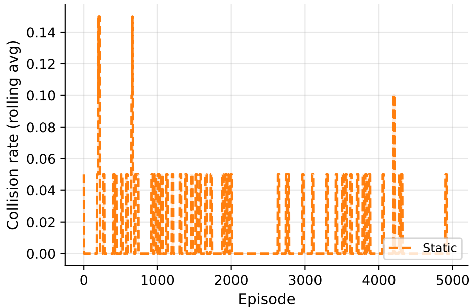
(b) Safety (collision rate)
