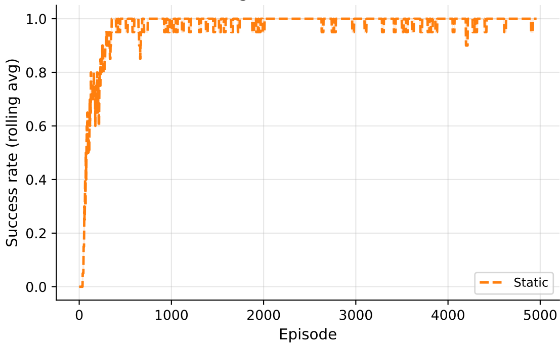
Learning curves — Success rate
