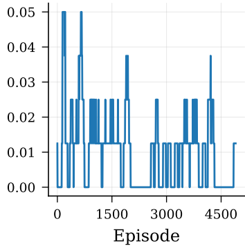
Collision Rate
