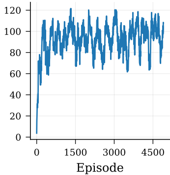
Episode Reward
