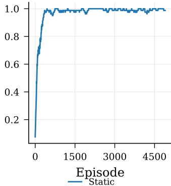
Success Rate
